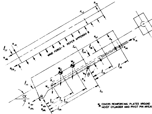
FIGURE 7—LOAD MOMENT DIAGRAM—BASE SECTION
