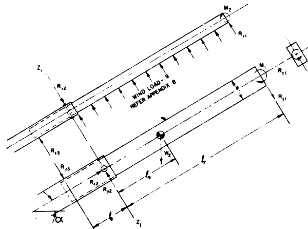
FIGURE 3—LOAD MOMENT DIAGRAM—TIP SECTION
