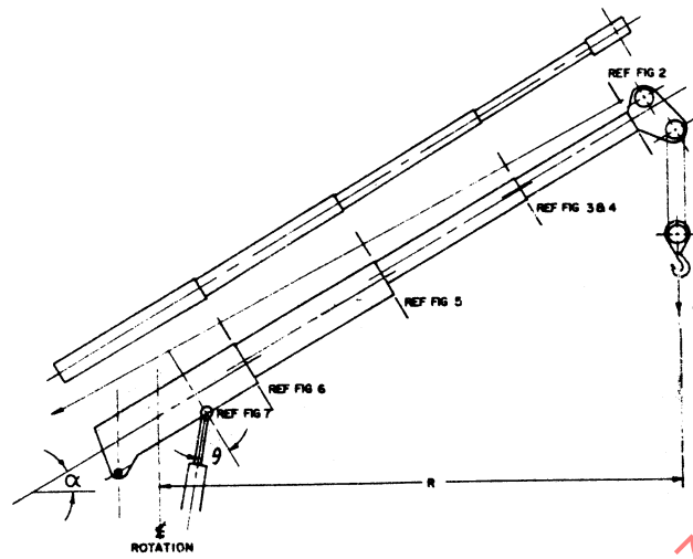
FIGURE 1—LOADING DIAGRAM—BOOM ASSEMBLY
