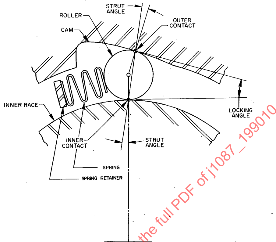
(R) FIGURE 1 - Outer Cam Type Loose Roller Clutch Diagram (Hook Type Cam)
