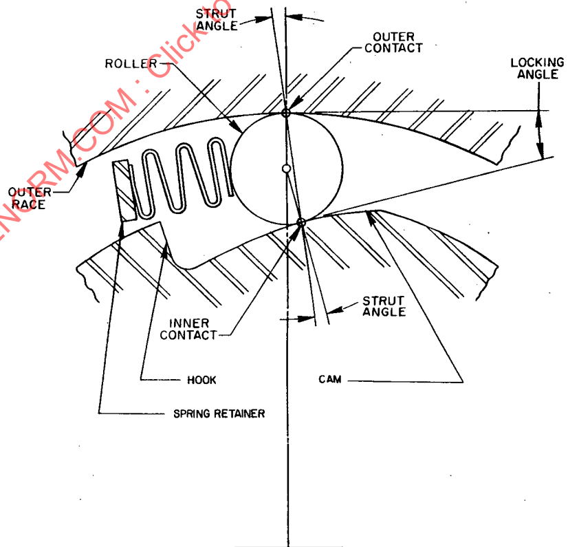
FIGURE 2 - Inner Cam Type Roller One-Way Clutch Diagram
