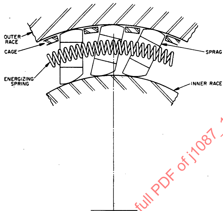
FIGURE 7 - Typical Single-Cage One-Way Clutch Diagram
