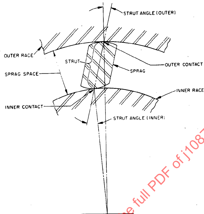
FIGURE 5 - Sprag One-Way Clutch Diagram
