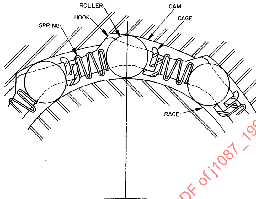
(R) FIGURE 3 - Caged Roller Outer Cam Type Clutch Diagram (Hook Type Cam)
