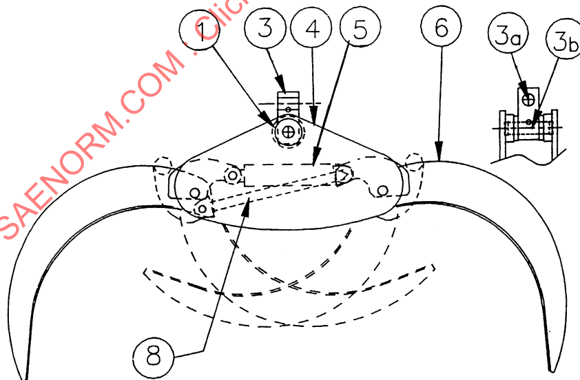
FIGURE 2—SINGLE CYLINDER CRADLE GRAPPLE
