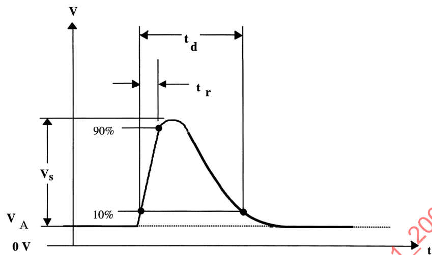
FIGURE 8 - TEST PULSE 5A LOAD DUMP, SINGLE PULSE - UNSUPPRESSED
