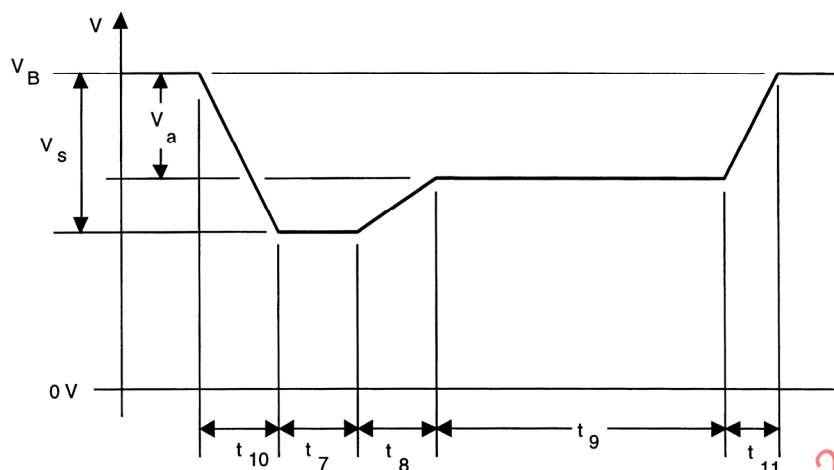
FIGURE 7 - TEST PULSE 4 SINGLE PULSE, i.e., STARTER MOTOR ENGAGEMENT DISTURBANCE
