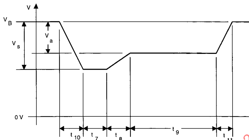
FIGURE 7 - TEST PULSE 4 SINGLE PULSE, i.e., STARTER MOTOR ENGAGEMENT DISTURBANCE
