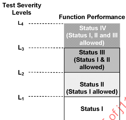
FIGURE B1 - FUNCTION PERFORMANCE STATUS CLASSIFICATION
