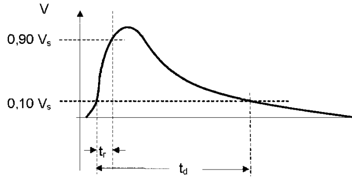
FIGURE C2 - DOUBLE EXPONENTIAL PULSE SHAPE GENERATED BY A TRANSIENT GENERATOR
