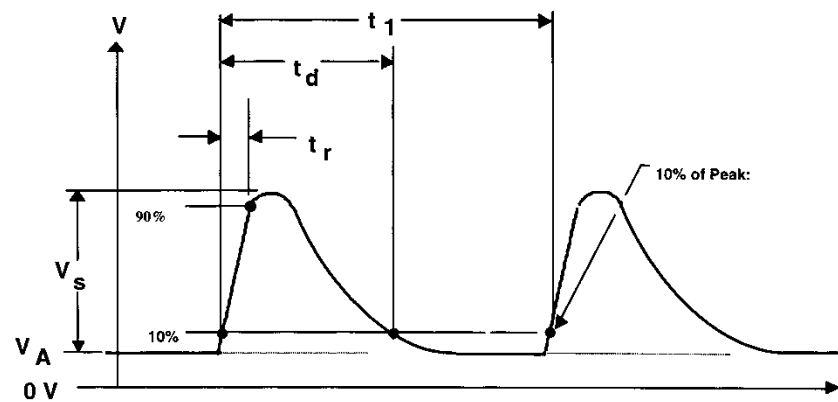
FIGURE 3 - TEST PULSE 2A SUDDEN INTERRUPTION OF CURRENT IN A DEVICE CONNECTED IN PARALLEL WITH THE DUT DUE TO THE WIRING HARNESS INDUCTANCE
