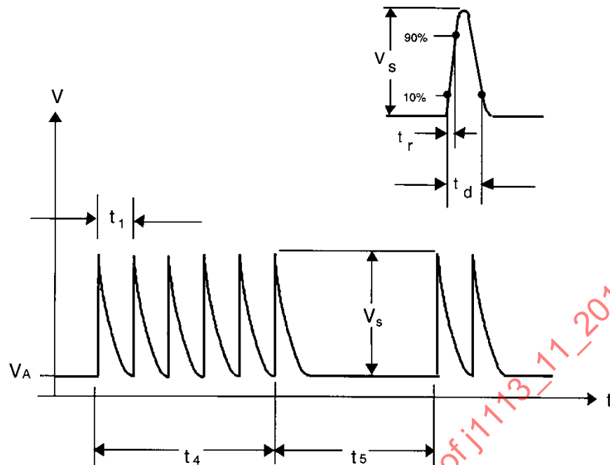
FIGURE 6 - TEST PULSE 3B SWITCHING SPIKES
