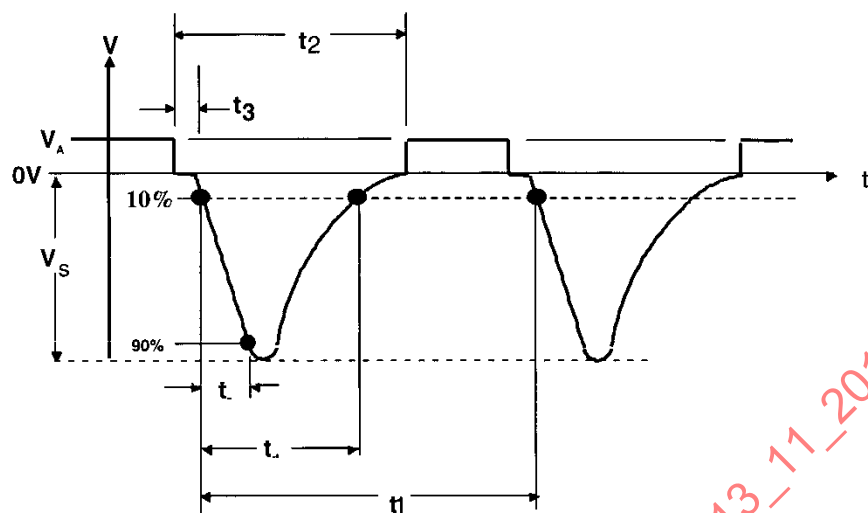
FIGURE 2 - TEST PULSE 1 SUPPLY DISCONNECTION FROM INDUCTIVE LOADS WITH DUT REMAINING CONNECTED DIRECTLY IN PARALLEL WITH THIS INDUCTIVE LOAD
