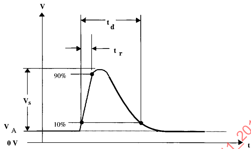
FIGURE 8 - TEST PULSE 5A & 5C LOAD DUMP, SINGLE PULSE - UNSUPPRESSED
