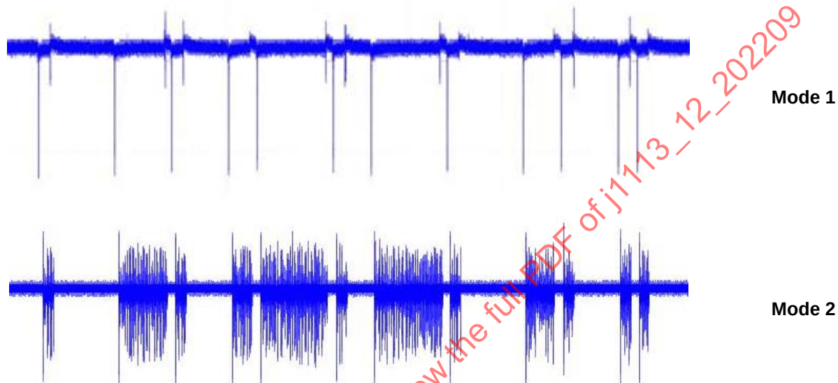
Figure 16 -Test mode characteristics
