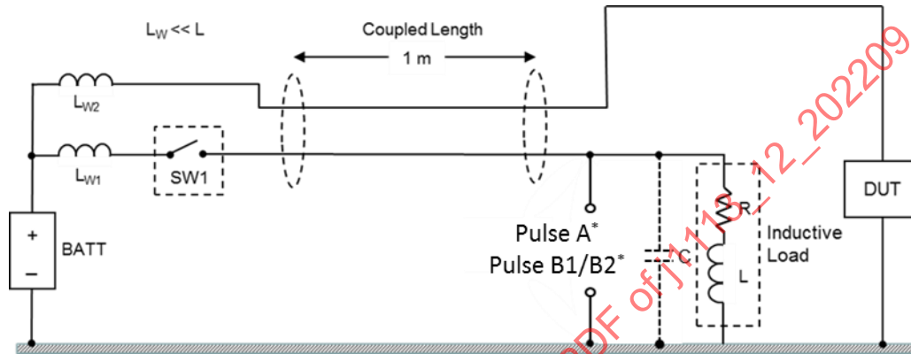
Figure 13 - Simplified automotive circuit for transient immunity
