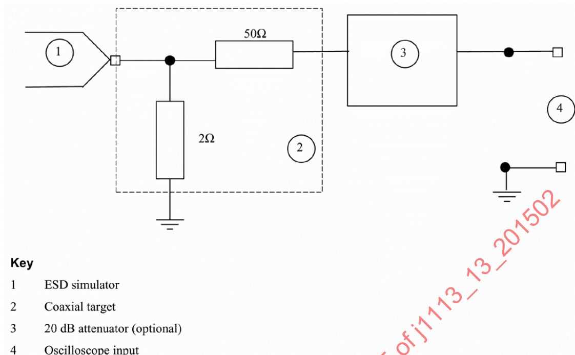
FIGURE A2—EQUIVALENT SCHEMATIC
