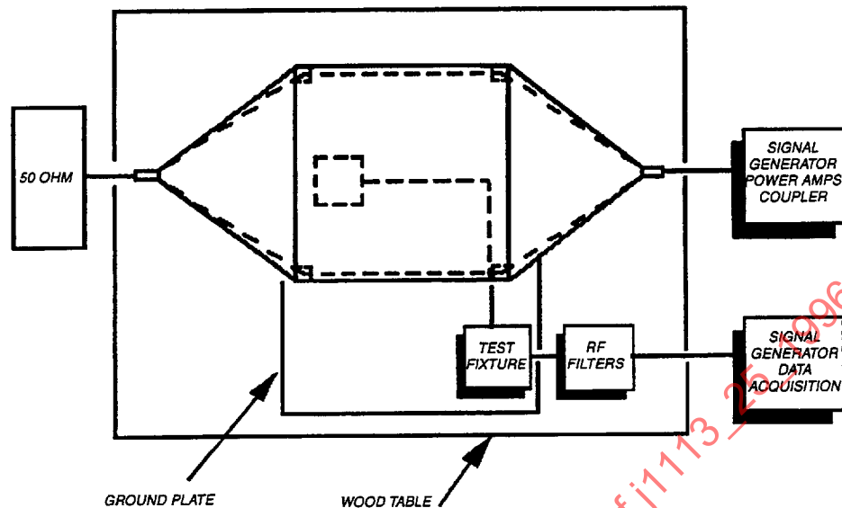
TRI-PLATE WITHIN ABSORBER LINED SHIELDED ROOM
