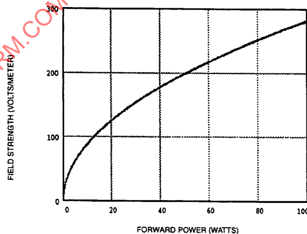
FIGURE A1—FIELD STRENGTH AS A FUNCTION OF FORWARD POWER
