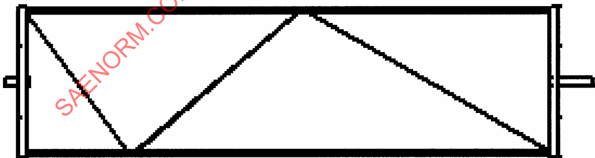
FIGURE A4—SIDE VIEW OF A Z-FOLD TUNER
