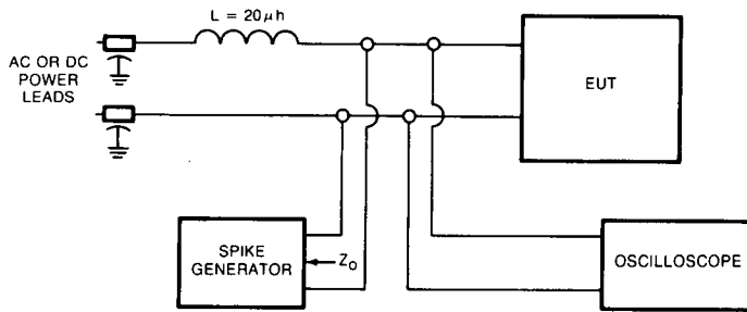
FIG. 10—TEST SETUP FOR CONDUCTED SUSCEPTIBILITY, SPIKE, POWER LEADS, INJECTION IN PARALLEL
