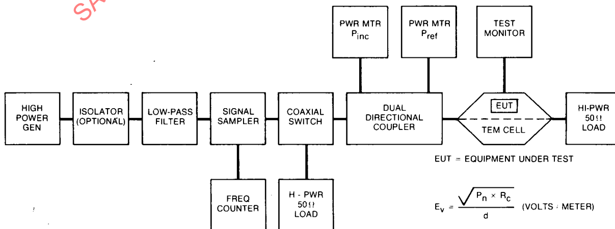
FIG. 17B—BLOCK DIAGRAM OF SYSTEM FOR SUSCEPTIBILITY TESTING OF EQUIPMENT (1 MHz–200 MHz)
