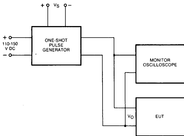
FIG. 11—TEST SETUP FOR CONDUCTED SUSCEPTIBILITY, LOAD DUMP AND FIELD DECAY, POWER LEADS
