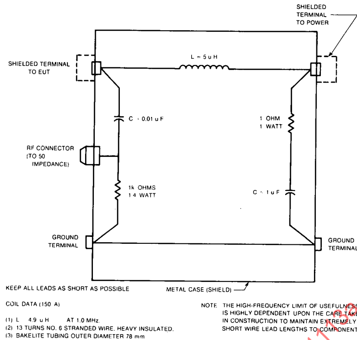
FIG. 4A—LINE IMPEDANCE STABILIZATION NETWORK (LISN), 5–100 MHz
