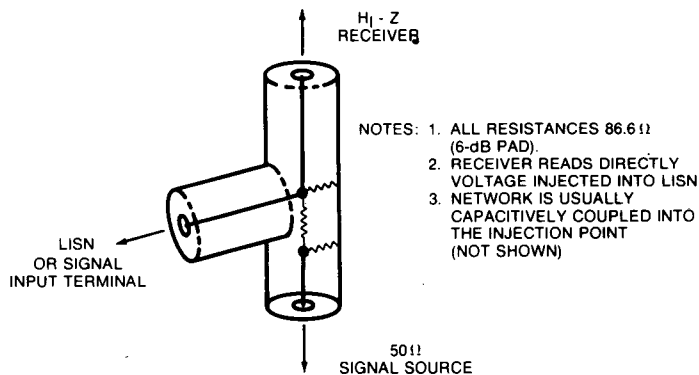
FIG. 5(B) - Z_G = 50 \Omega , Z_R \gg 50 \Omega
