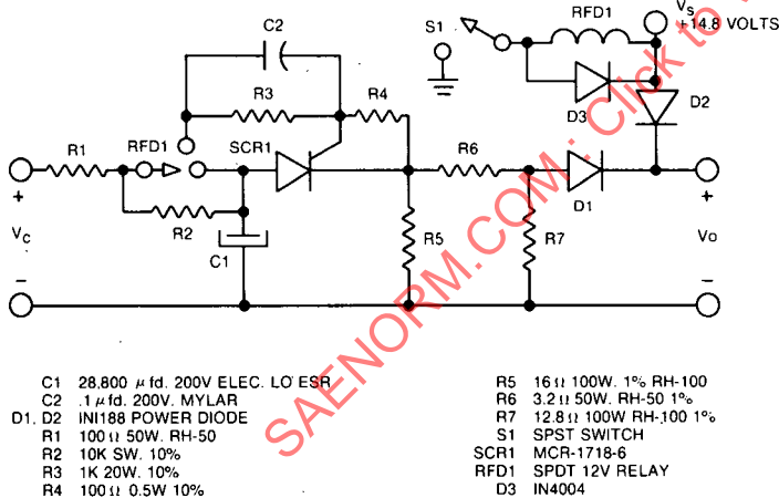
FIG. 12—TYPICAL LOAD DUMP TRANSIENT SIMULATOR
