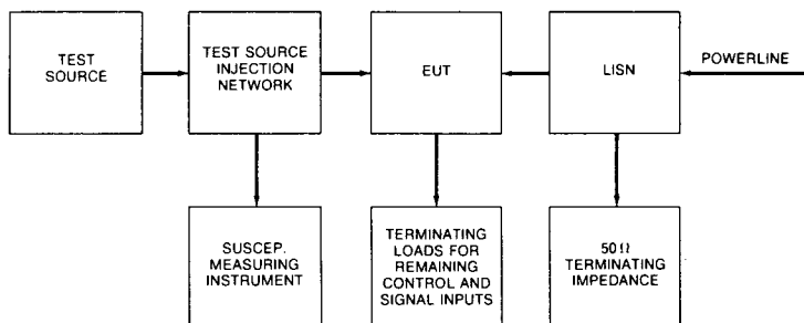
FIG. 7 - EQUIPMENT BLOCK DIAGRAM FOR MEASURING CONDUCTED SUSCEPTIBILITY 50 kHz - 100 MHz, CONTROL AND SIGNAL INPUTS
