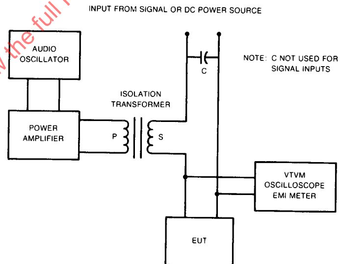
FIG. 1—TEST SETUP FOR MEASURING CONDUCTED SUSCEPTIBILITY, 30 Hz–50 kHz, SIGNAL OR DC POWER INPUT
