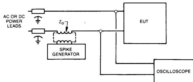
FIG. 9 - TEST SETUP FOR CONDUCTED SUSCEPTIBILITY, SPIKE, POWER LEADS, INJECTION IN SERIES
