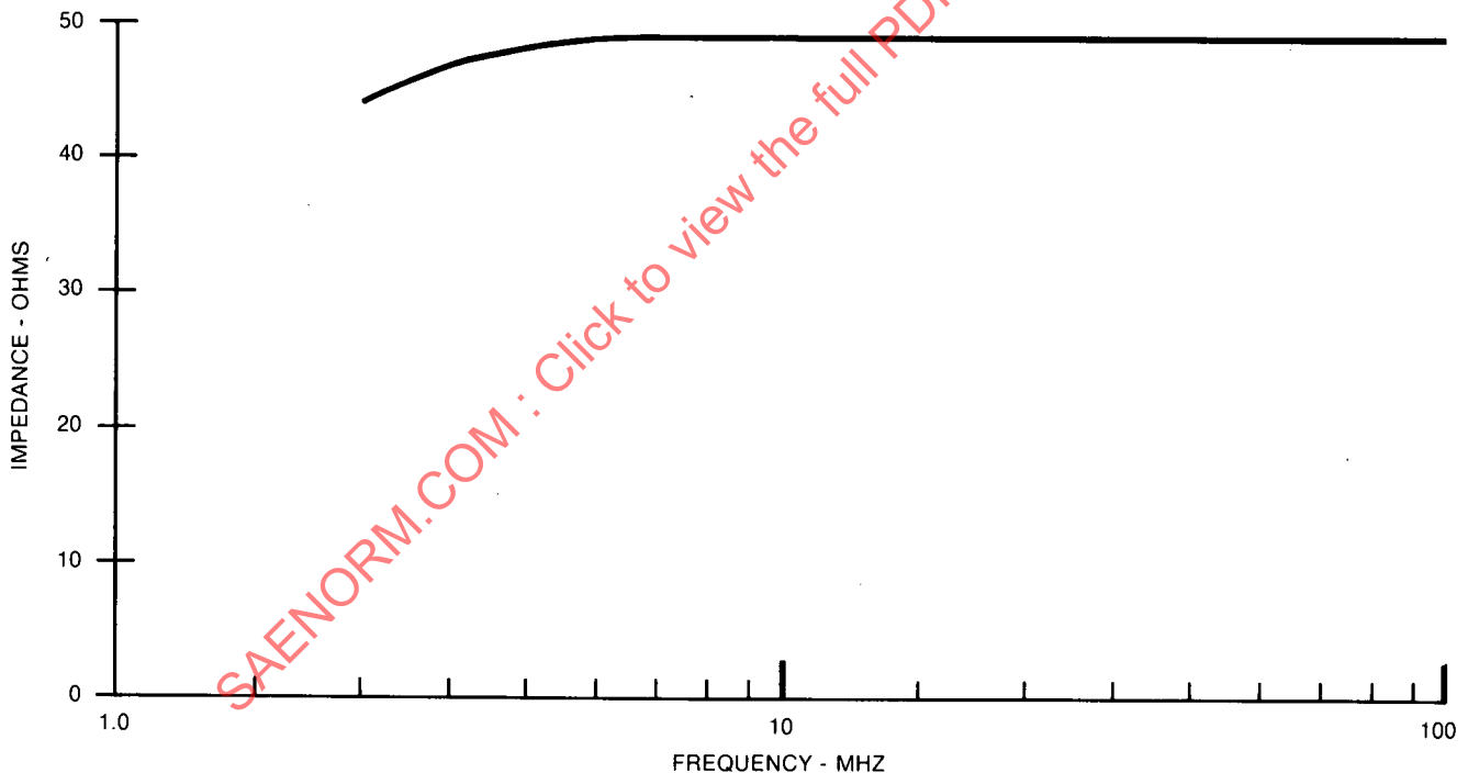
FIG. 4B—LINE IMPEDANCE STABILIZATION NETWORK REFERENCE IMPEDANCE, 5–100 MHz
