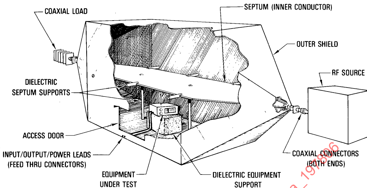
FIG. 16—CUT-AWAY VIEW OF TEM CELL BEING USED FOR EM SUSCEPTIBILITY TESTING. FIGURE SHOWS PLACEMENT OF EUT AND ASSOCIATED INPUT, OUTPUT, AND MONITORING LEADS INSIDE THE CELL
