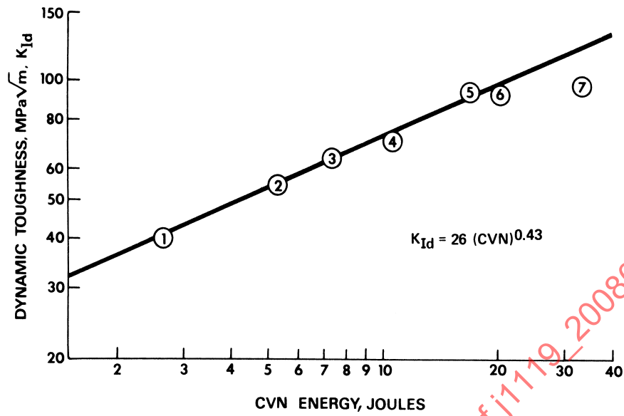
FIGURE 5—CVN—K1D CORRELATION
