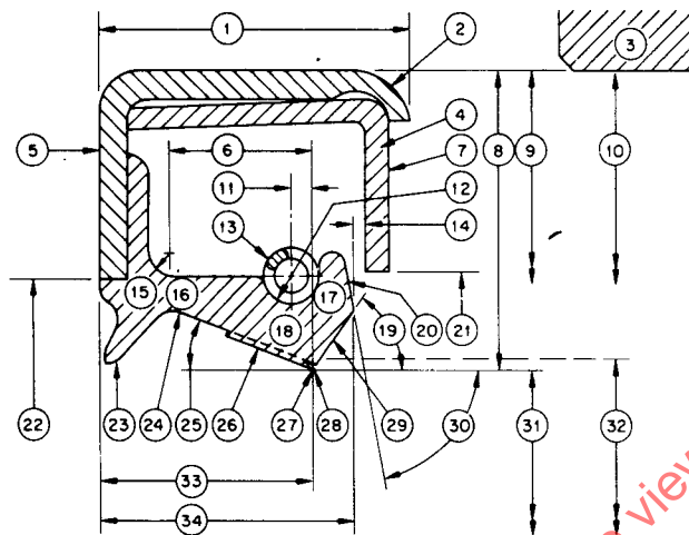
FIG. 1—NOMENCLATURE FOR DETAILS OF RADIAL LIP SEAL
