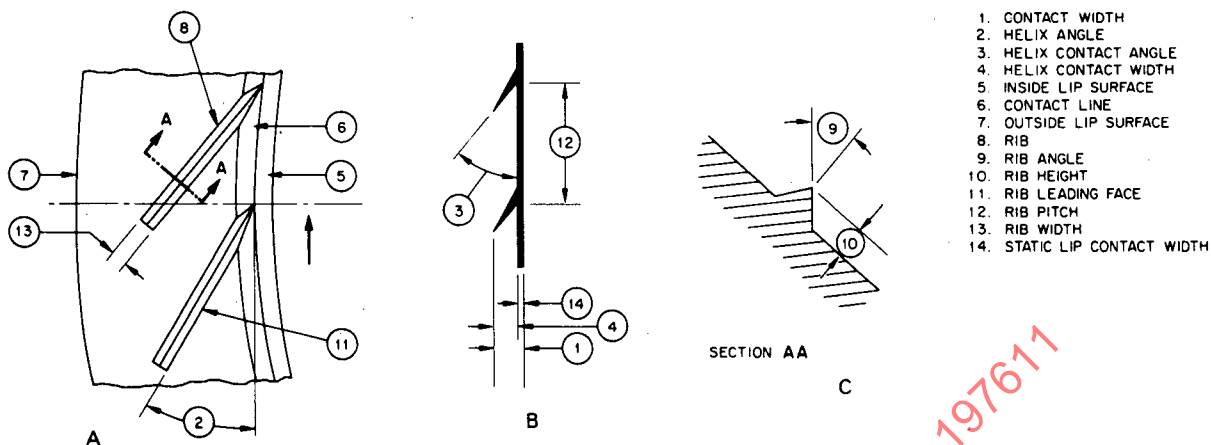
FIG. 2—NOMENCLATURE FOR OUTER LIP SURFACE AND CONTACT SURFACE. DETAILS OF RADIAL LIP SEAL (HELIX SEAL TYPE): (A) VIEW IN PLANE OF OUTSIDE LIP SURFACE, (B) VIEW OF CONTACT SURFACE, (C) CROSS SECTION OF RIB
