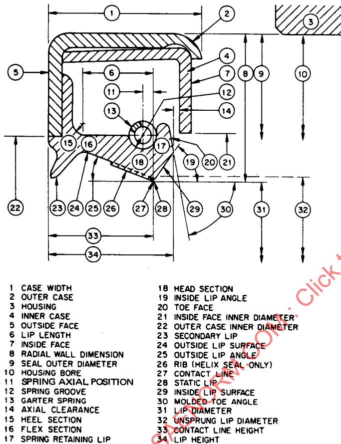
FIG. 1—NOMENCLATURE FOR DETAILS OF RADIAL LIP SEAL
