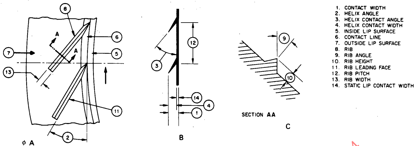
FIG. 2—NOMENCLATURE FOR OUTER LIP SURFACE AND CONTACT SURFACE. DETAILS OF RADIAL LIP SEAL (HELIX SEAL TYPE): (A) VIEW IN PLANE OF OUTSIDE LIP SURFACE, (B) VIEW OF CONTACT SURFACE, (C) CROSS SECTION OF RIB
