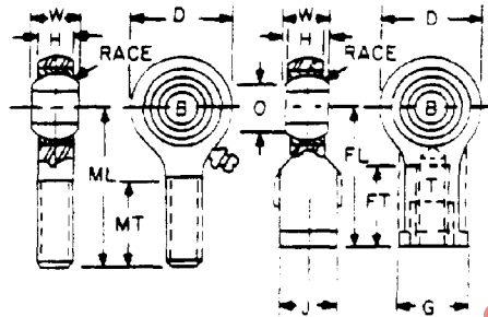
FIGURE 2—TYPE A METALLIC RACE
