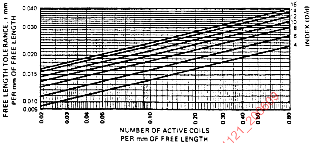
FIGURE 5—FREE LENGTH TOLERANCE - COMPRESSION SPRINGS. ROUND OFF INDEX TO NEAREST WHOLE NUMBER. INTERPOLATE WHEN ROUNDED-OFF VALUE IS ODD NUMBER. THESE ARE TOLERANCES FOR SPRINGS WITH ENDS CLOSED AND GROUND. FOR SPRINGS WITH ENDS CLOSED BUT NOT GROUND, MULTIPLY BY 1.7.
