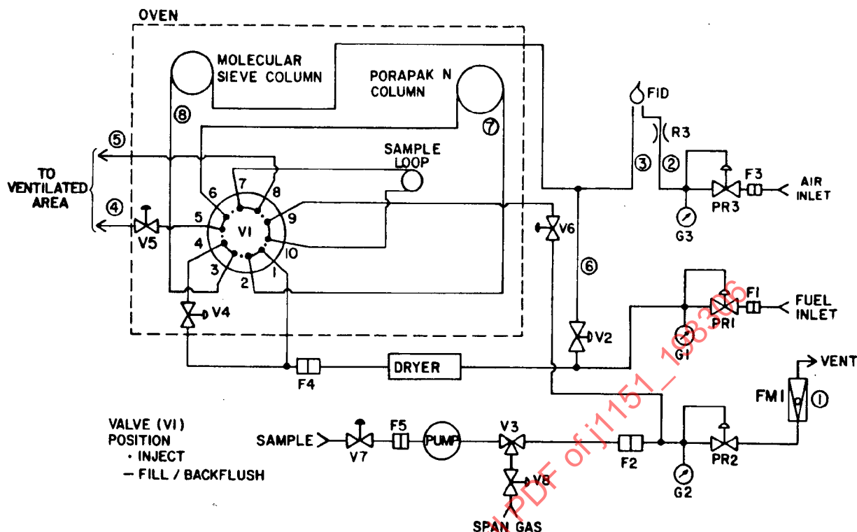
FIG. 1—INSTRUMENT TO MEASURE METHANE
