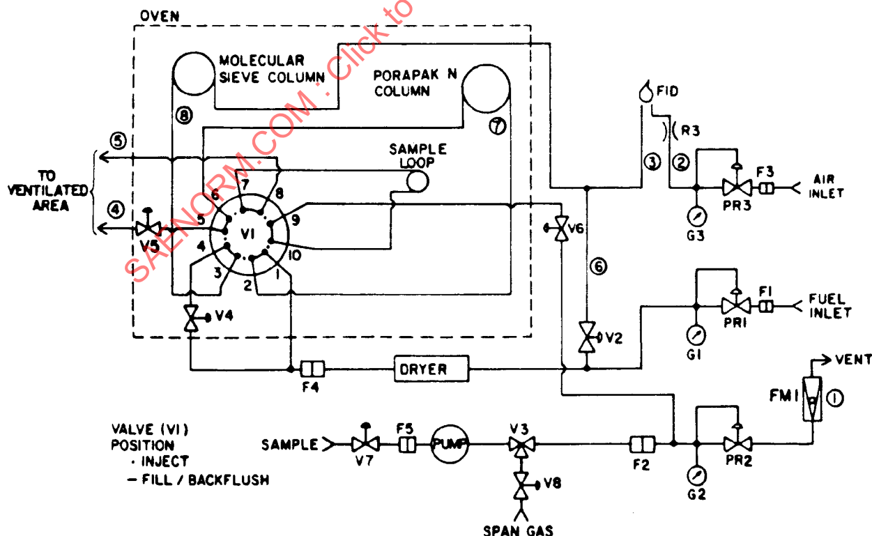
FIGURE 1 - Instrument to Measure Methane
