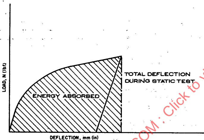
FIG. 8—FORCE DEFLECTION (F-D) CURVE
