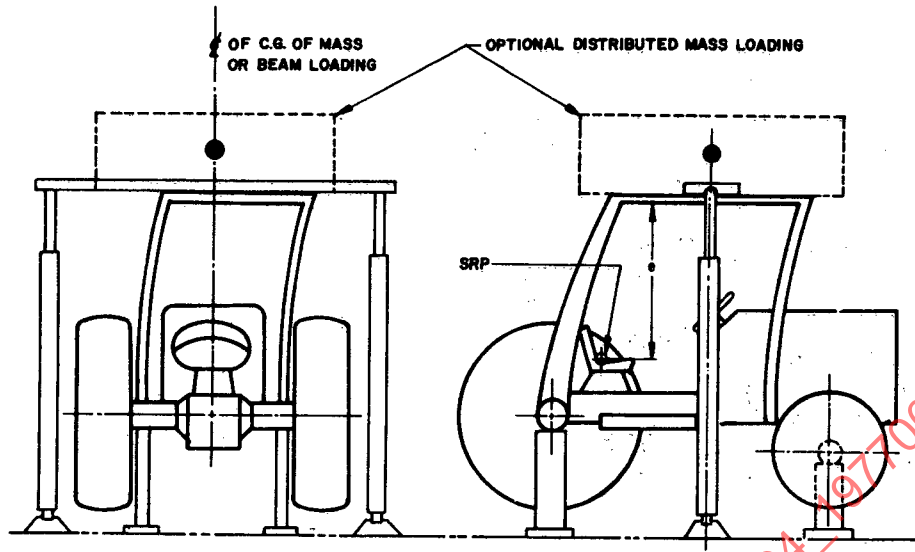
FIG. 7—TYPICAL METHOD OF LOAD APPLICATION FOR CRUSH TEST
