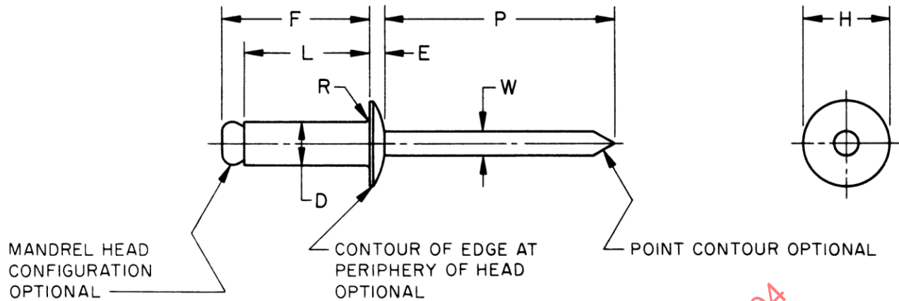
FIGURE 4—REGULAR AND LARGE PROTRUDING HEAD STYLE MANDREL BLIND RIVET DETAIL (SEE Tables 6A AND 6B)
