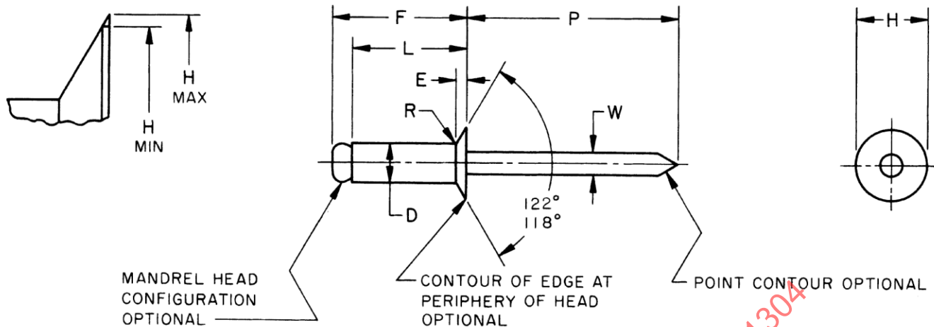
FIGURE 5—120 DEGREE COUNTERSUNK FLUSH HEAD STYLE BREAK MANDREL BLIND RIVET DETAIL (SEE Tables 7A AND 7B)
