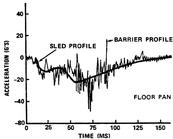
FIGURE 6—48 KM/H (30 MPH) BARRIER AND SLED SHOCK PROFILES
