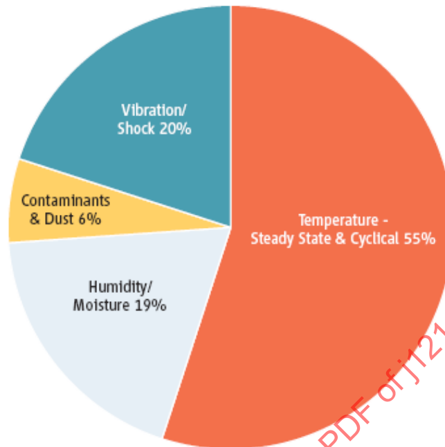
FIGURE 17 - SOURCES OF STRESS FOR ELECTRONIC EQUIPMENT
