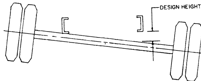
FIGURE 6A—SOLID AXLE REAR SUSPENSION TRAVEL—ONE WHEEL JOUNCE
