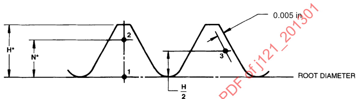
FIGURE 2—POSITIONS FOR DETERMINING HARDNESS
