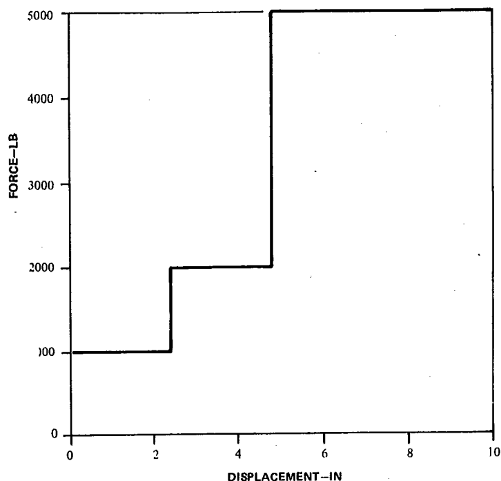
FIG. 2—NOMINAL DECELERATOR CHARACTERISTICS
