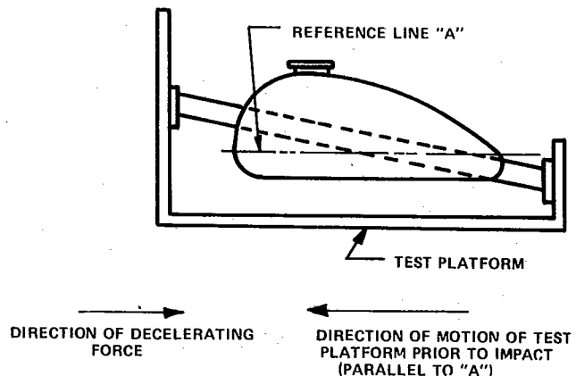
FIG. 1—FUEL TANK POSITION FOR LONGITUDINAL ACCELERATION TEST
