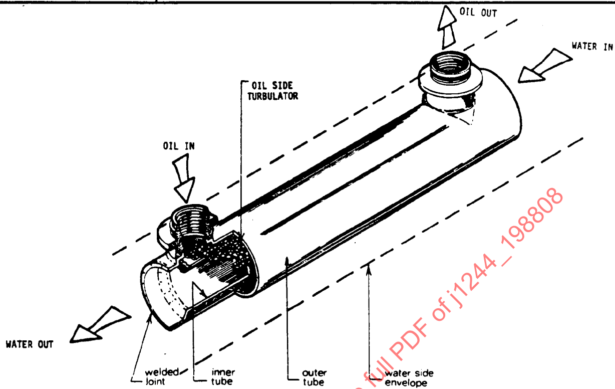
FIGURE 5 - Concentric Tube Oil to Water Cooler
