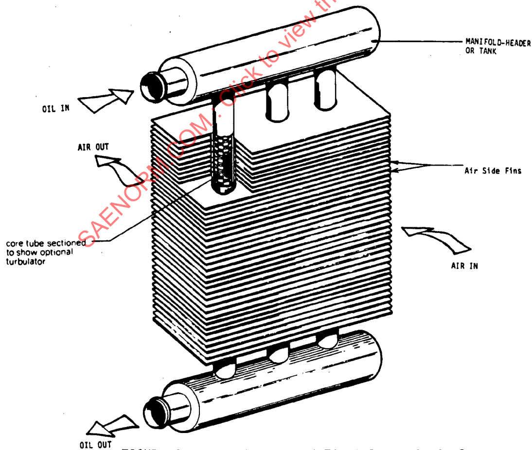
FIGURE 6A - Round Tube and Fin Oil to Air Cooler
