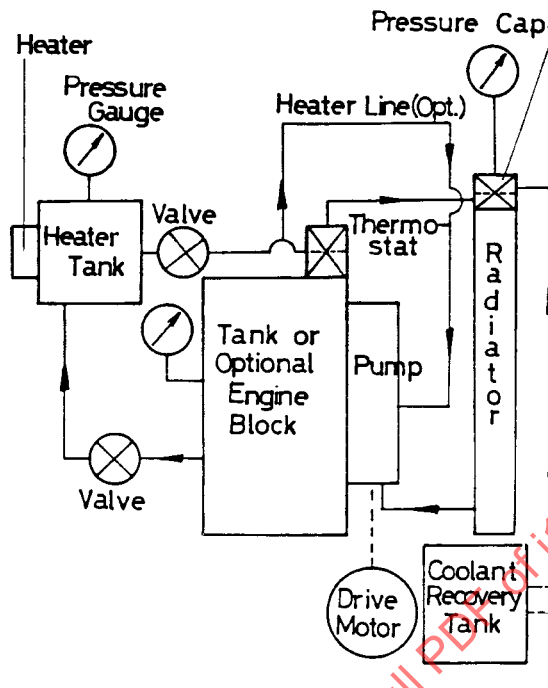
FIGURE 2—SCHEMATIC—ENGINE COOLANT PUMP SEAL DURABILITY TEST SYSTEM
