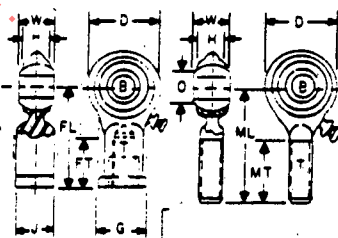
FIGURE 4 - Type C - Raceless
