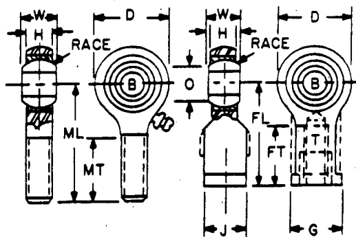
FIGURE 2 - Type A - Metallic Race
