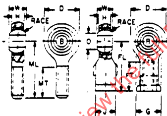
FIGURE 3 - Type B - Molded Race
