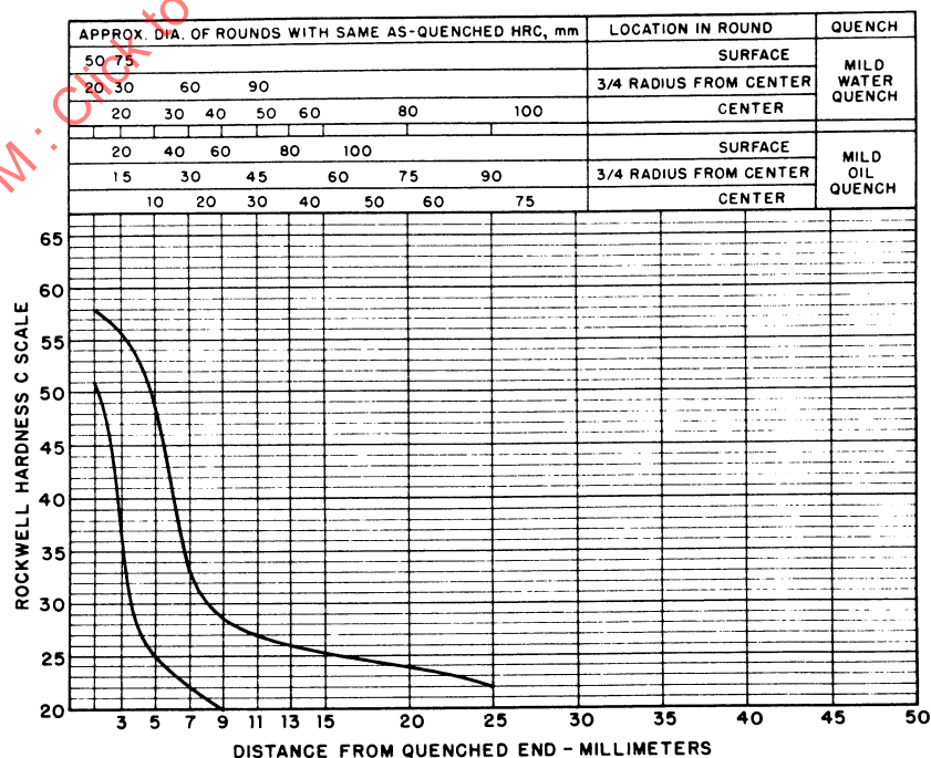
FIGURE 3—UNS H10380—HARDENABILITY BAND—SAE 1038H
