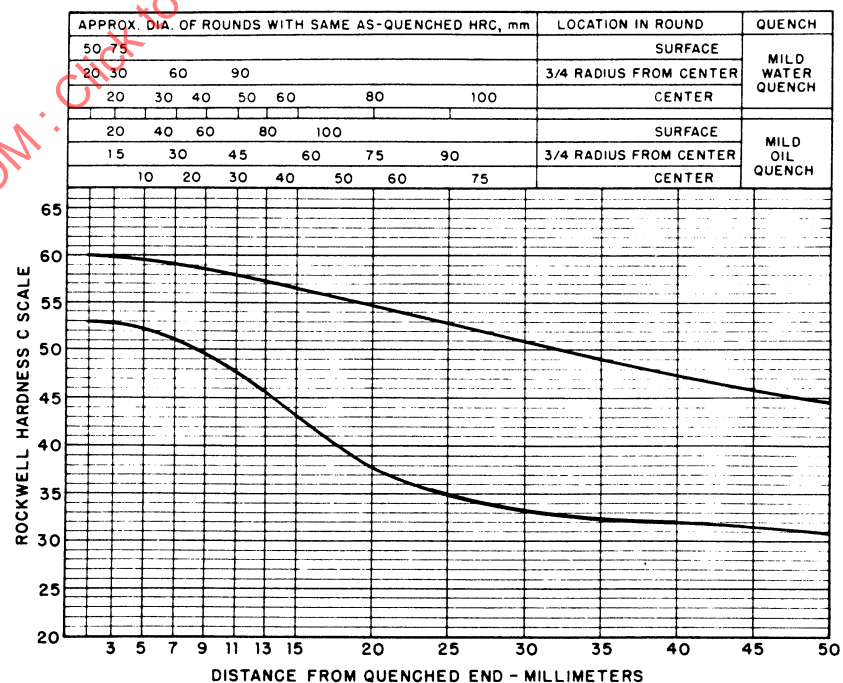
FIGURE 31—UNS H41400—HARDENABILITY BAND—4140H
