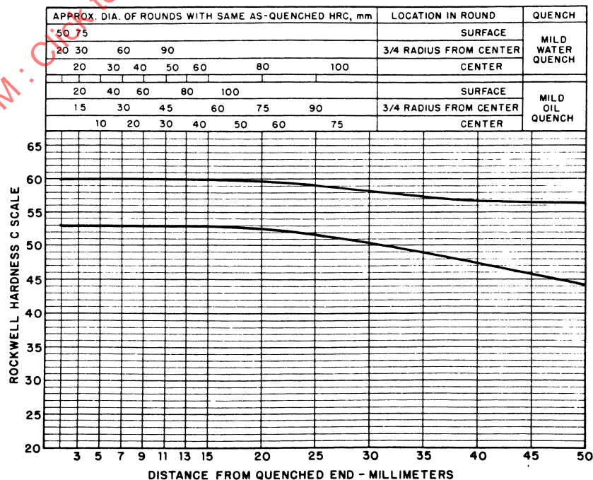
FIGURE 39—UNS H43406—HARDENABILITY BAND—SAE E4340H
