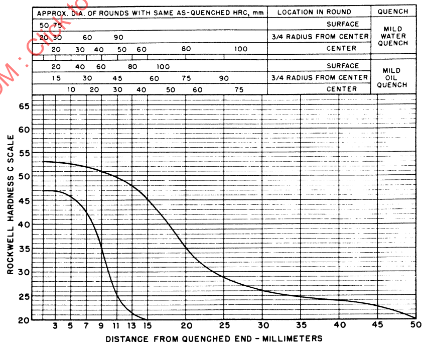
FIGURE 10—UNS H15281—HARDENABILITY BAND—SAE 15B28H
