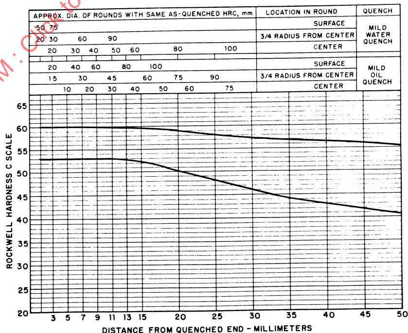
FIGURE 38—UNS H43400—HARDENABILITY BAND—SAE 4340H
