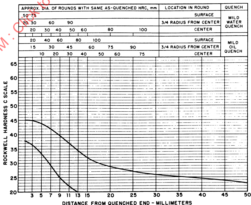
FIGURE 43—UNS H48150—HARDENABILITY BAND—SAE 4815H
