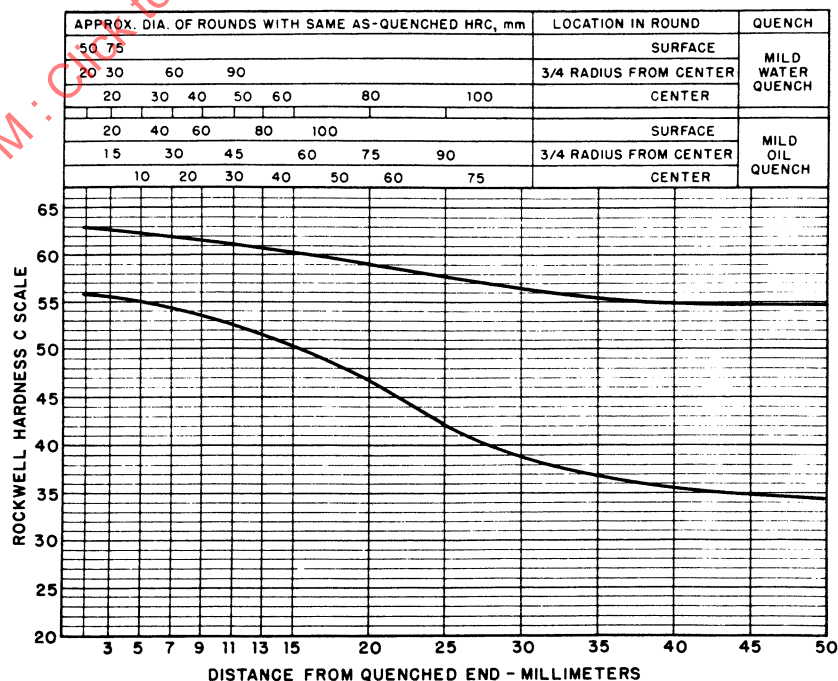
FIGURE 33—UNS H41450—HARDENABILITY BAND—SAE 4145H
