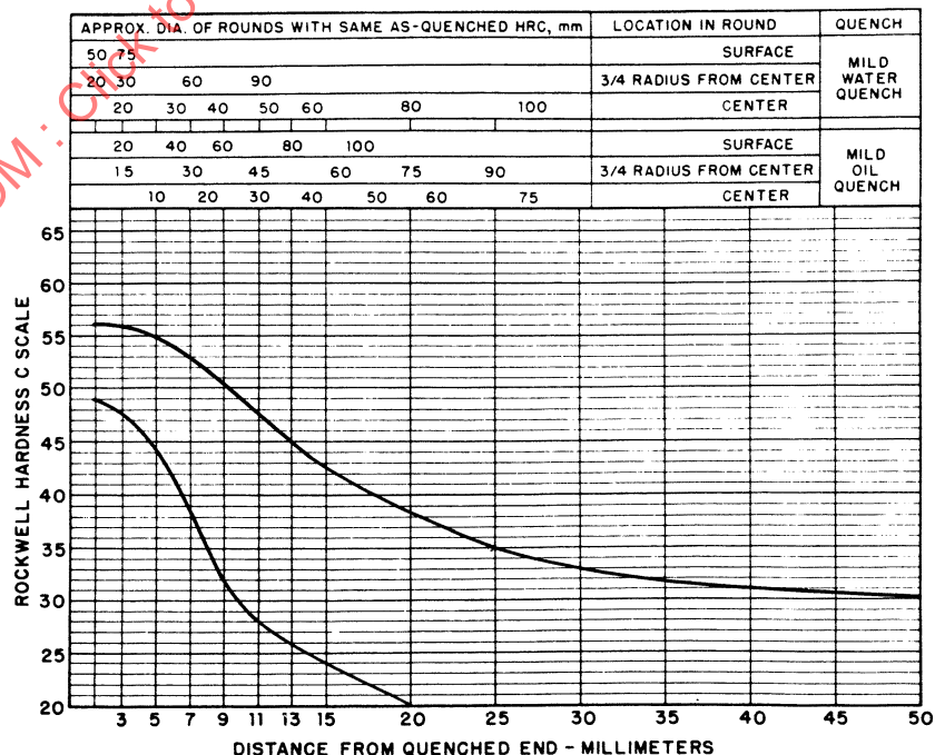
FIGURE 17—UNS H13300—HARDENABILITY BAND—SAE 1330H
