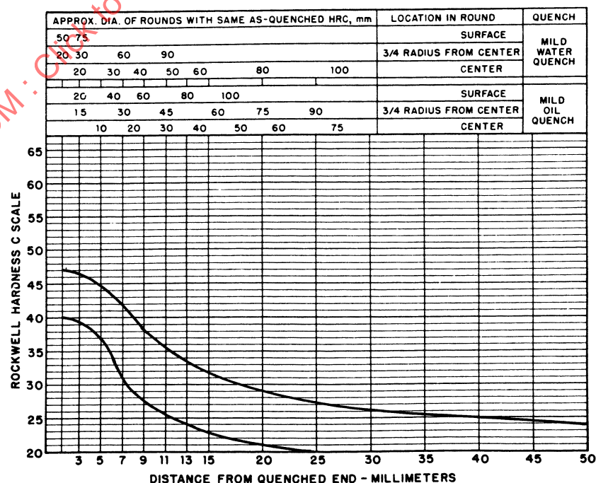
FIGURE 41—UNS H47180—HARDENABILITY BAND—SAE 4718H
