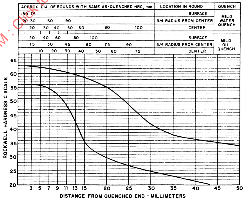
FIGURE 47—UNS H50441—HARDENABILITY BAND—SAE 50B44H
