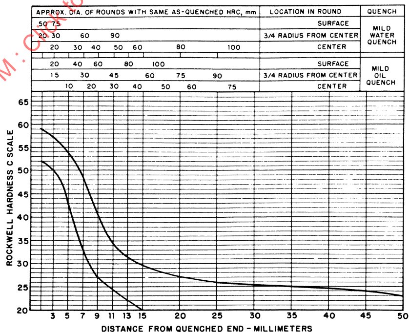
FIGURE 23—UNS H40370—HARDENABILITY BAND—SAE 4037H
