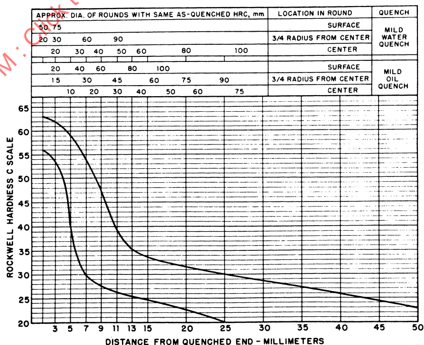
FIGURE 48—UNS H50460—HARDENABILITY BAND—SAE 5046H
