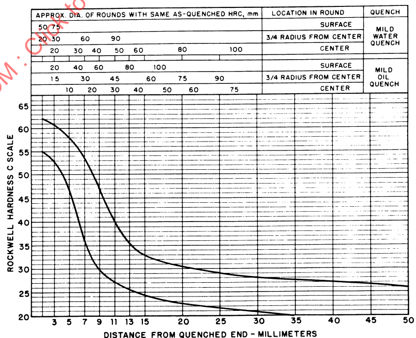
FIGURE 24—UNS H40420—HARDENABILITY BAND—SAE 4042H
