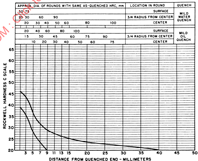
FIGURE 62—UNS H61180—HARDENABILITY BAND—SAE 6118H
