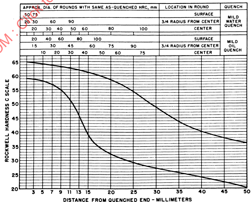
FIGURE 50—UNS H50501—HARDENABILITY BAND—SAE 50B50H
