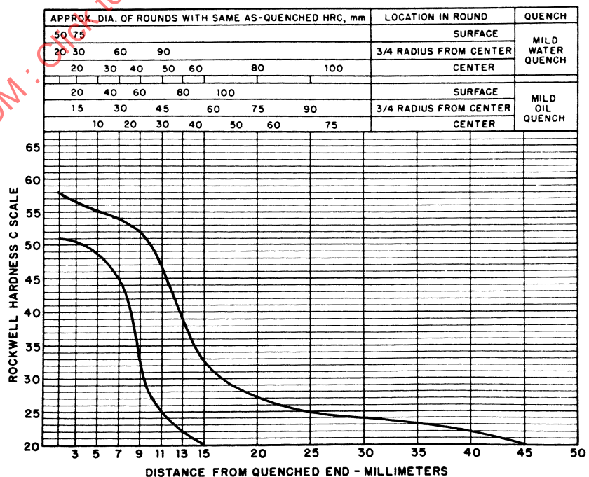
FIGURE 12—UNS H15351—HARDENABILITY BAND—SAE 15B35H
