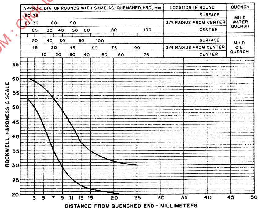
FIGURE 8—UNS H15410—HARDENABILITY BAND—SAE 1541H
