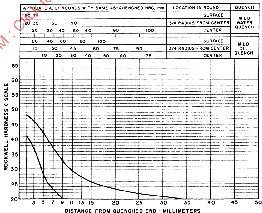
FIGURE 40—UNS H46200—HARDENABILITY BAND—SAE 4620H
