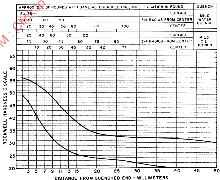
FIGURE 28—UNS H41300—HARDENABILITY BAND—SAE 4130H
