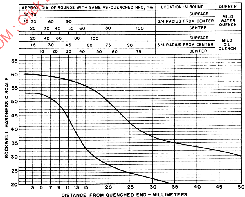
FIGURE 46—UNS H50401—HARDENABILITY BAND—SAE 50B40H
