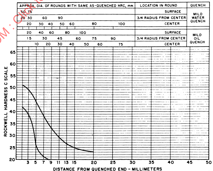
FIGURE 6—UNS H15240—HARDENABILITY BAND—SAE 1524H
