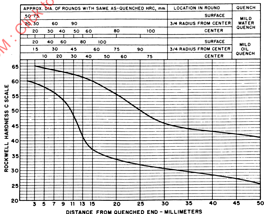
FIGURE 59—UNS H51550—HARDENABILITY BAND—SAE 5155H
