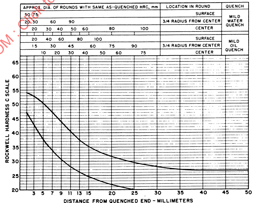
FIGURE 69—UNS H86270—HARDENABILITY BAND—SAE H8627H
