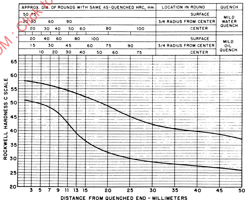
FIGURE 29—UNS H41350—HARDENABILITY BAND—SAE 4135H
