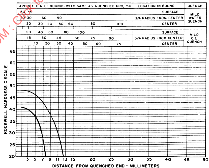
FIGURE 9—UNS H15211—HARDENABILITY BAND—SAE 15B21H
