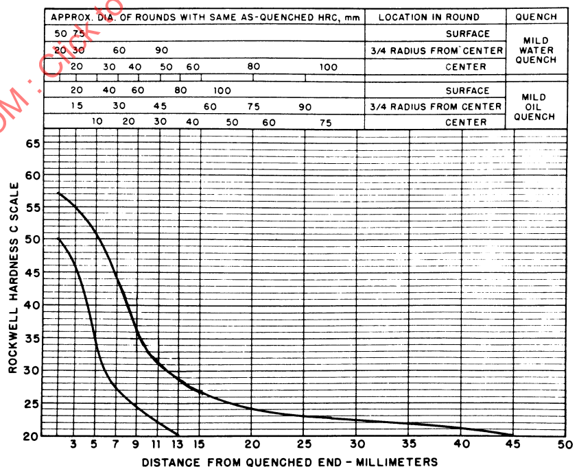
FIGURE 22—UNS H40320—HARDENABILITY BAND—SAE 4032H
