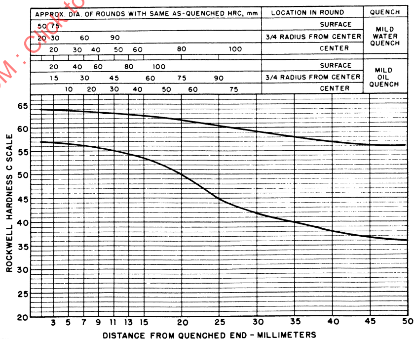
FIGURE 34—UNS H41470—HARDENABILITY BAND—SAE 4147H
