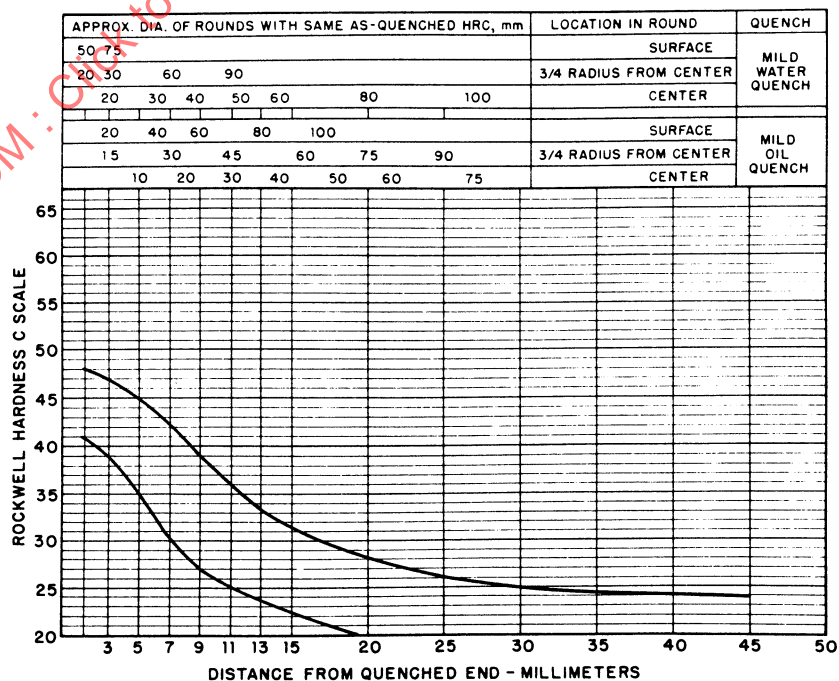
FIGURE 37—UNS H43200—HARDENABILITY BAND—SAE 4320H
