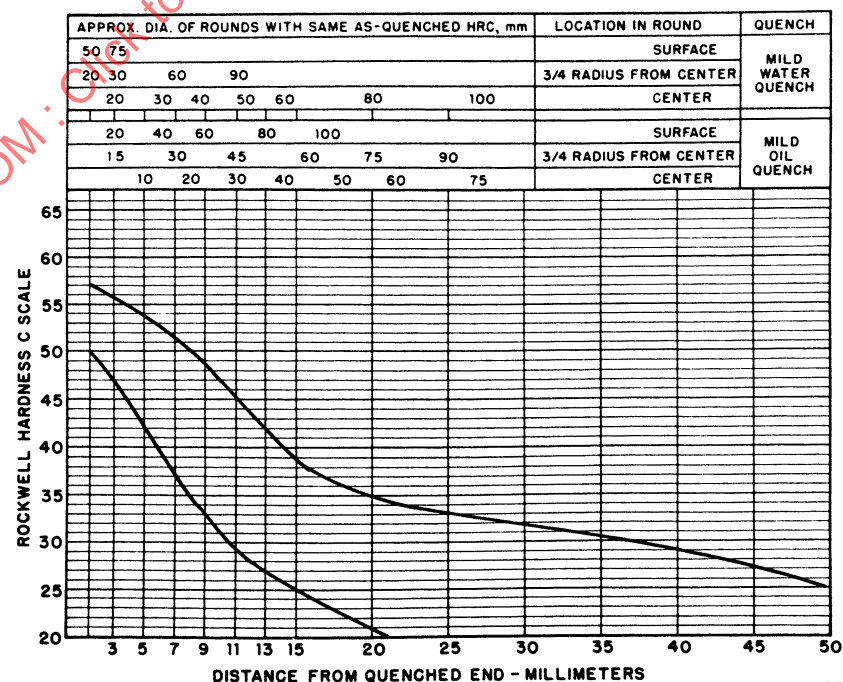
FIGURE 54—UNS H51320—HARDENABILITY BAND—SAE 5132H
