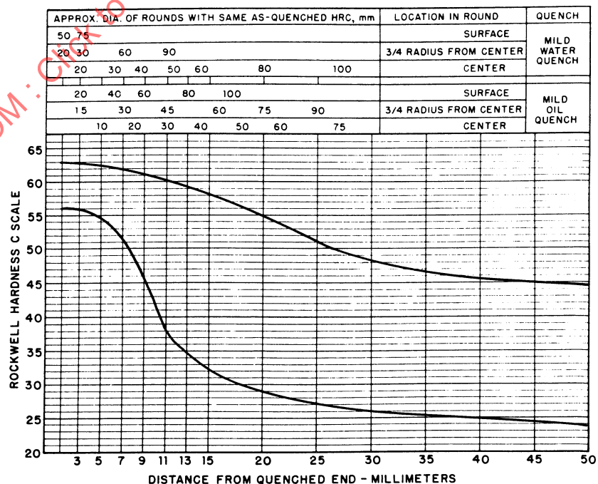
FIGURE 20—UNS H13450—HARDENABILITY BAND—SAE 1345H
