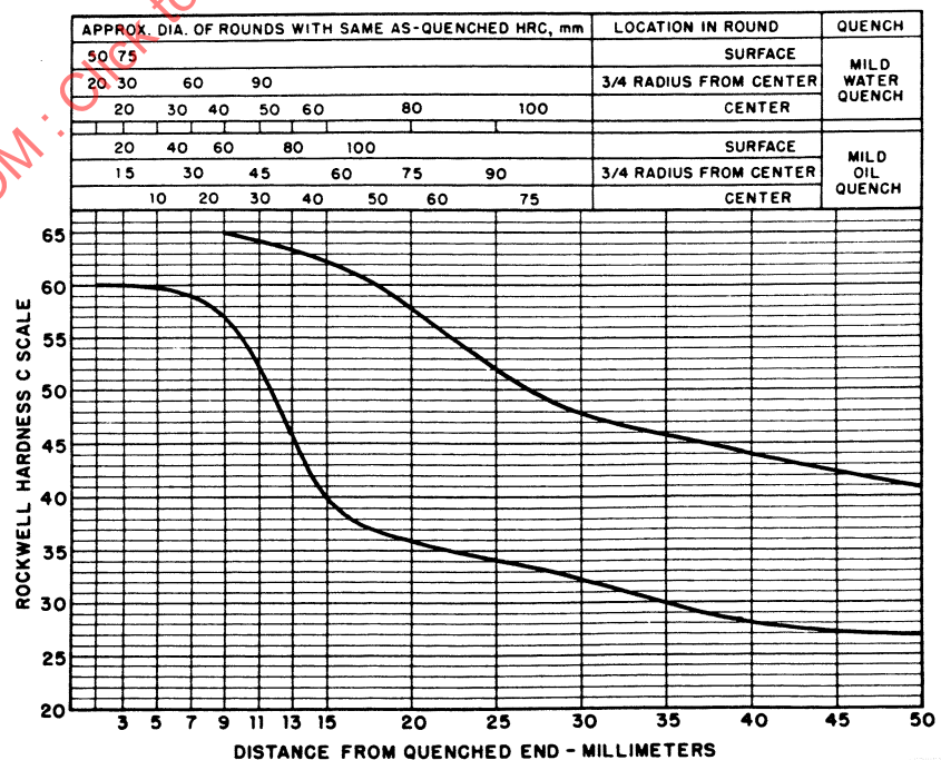
FIGURE 60—UNS H51600—HARDENABILITY BAND—SAE 5160H
