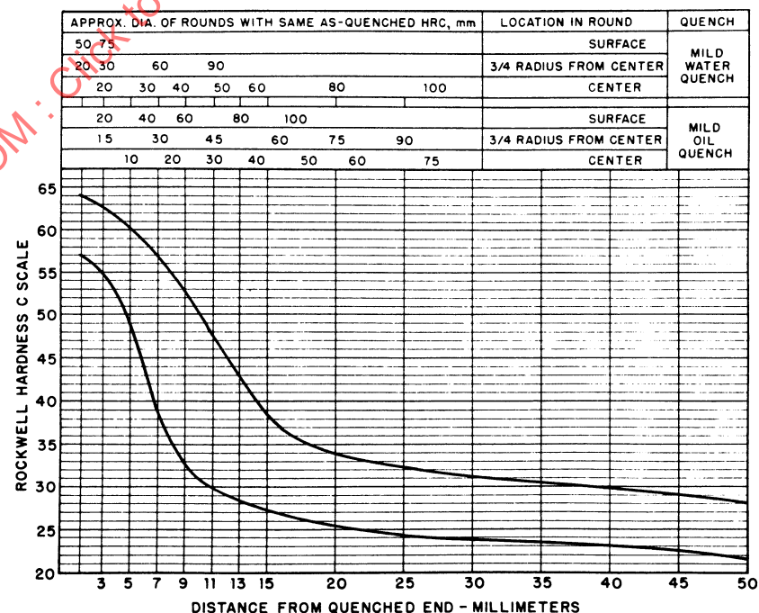
FIGURE 25—UNS H40470—HARDENABILITY BAND—SAE 4047H
