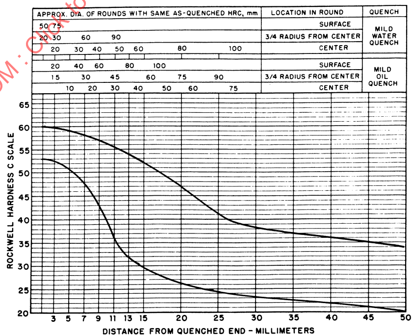
FIGURE 19—UNS H13400—HARDENABILITY BAND—SAE 1340H
