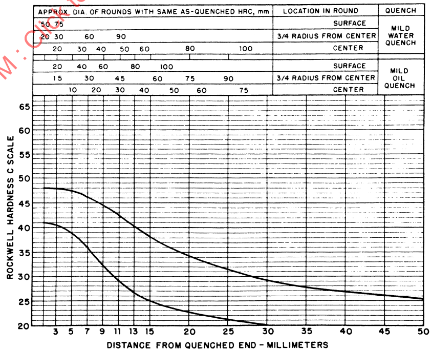
FIGURE 45—UNS H48200—HARDENABILITY BAND—SAE 4820H
