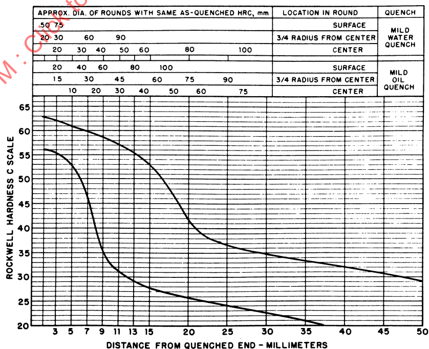
FIGURE 49—UNS H50461—HARDENABILITY BAND—SAE 50B46H
