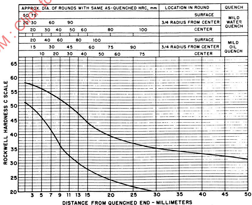
FIGURE 55—UNS H51350—HARDENABILITY BAND—SAE 5135H
