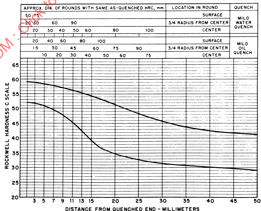
FIGURE 30—UNS 41370—HARDENABILITY BAND—SAE 4137H
