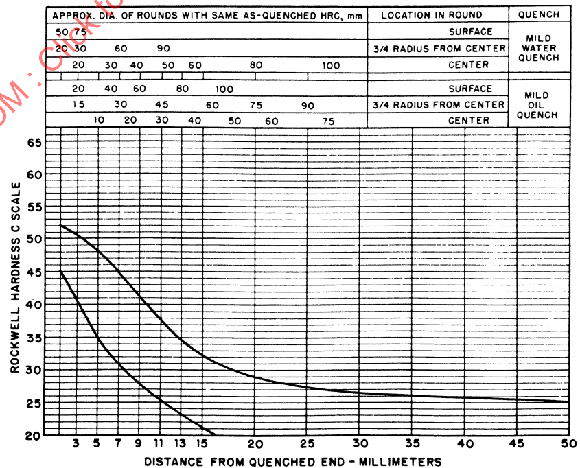
FIGURE 68—UNS H86250—HARDENABILITY BAND—SAE 8625H
