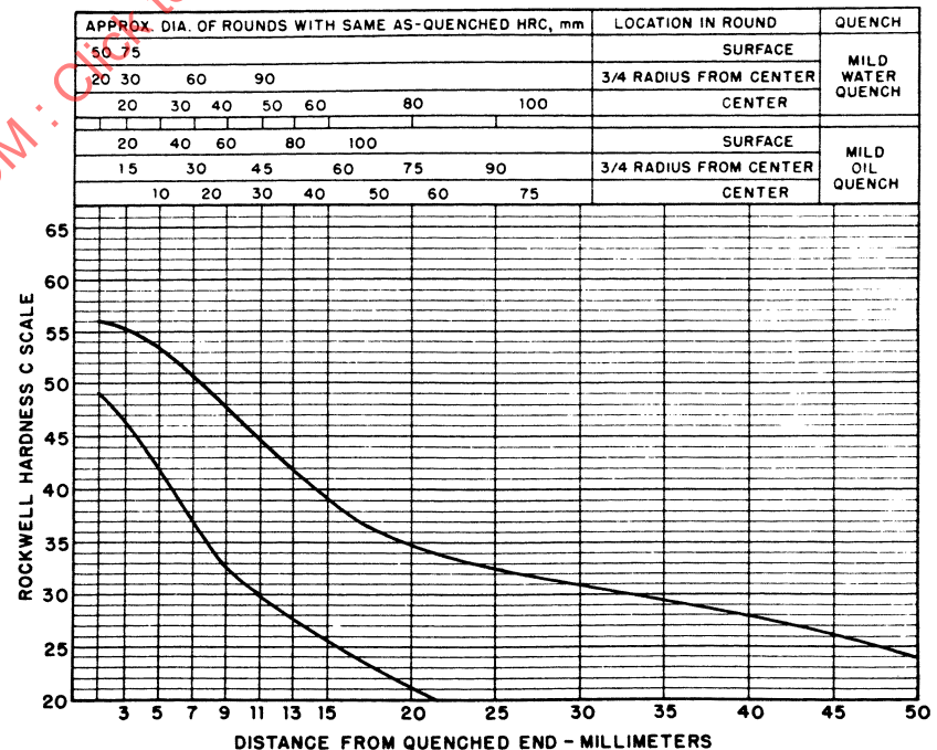
FIGURE 53—UNS H51300—HARDENABILITY BAND—SAE 5130H
