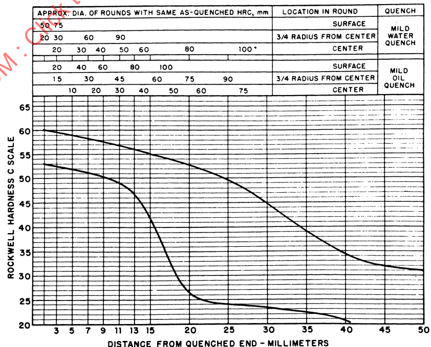
FIGURE 14—UNS H15411—HARDENABILITY BAND—SAE 15B41H
