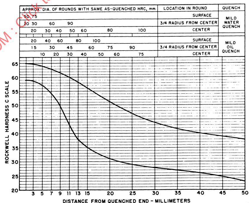
FIGURE 58—UNS H51500—HARDENABILITY BAND—SAE 5150H
