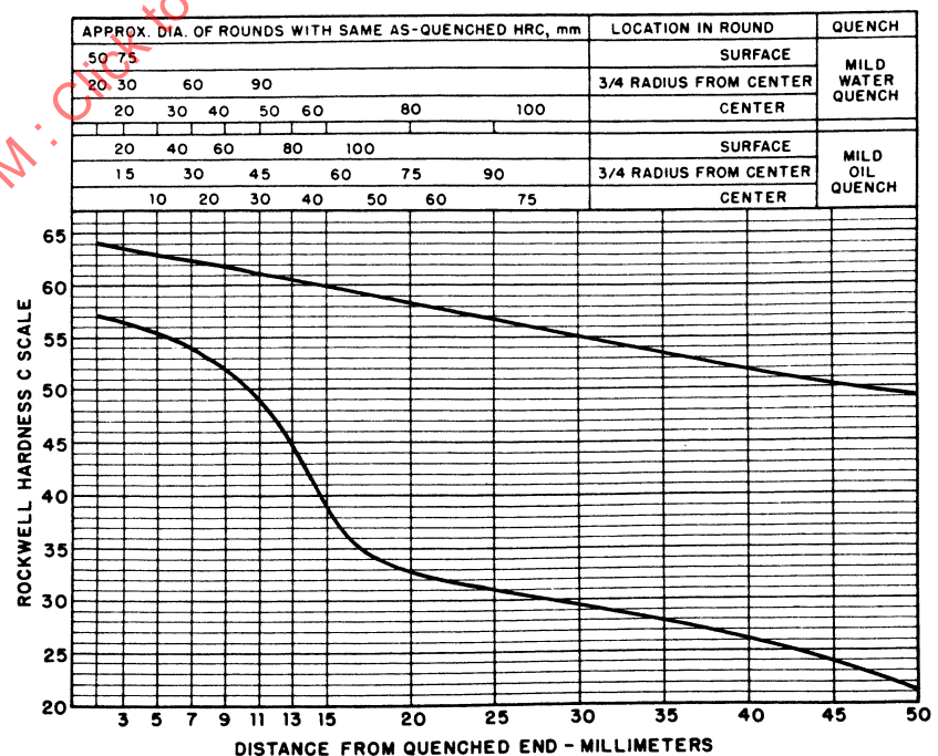
FIGURE 57—UNS 51470—HARDENABILITY BAND—SAE 5147H
