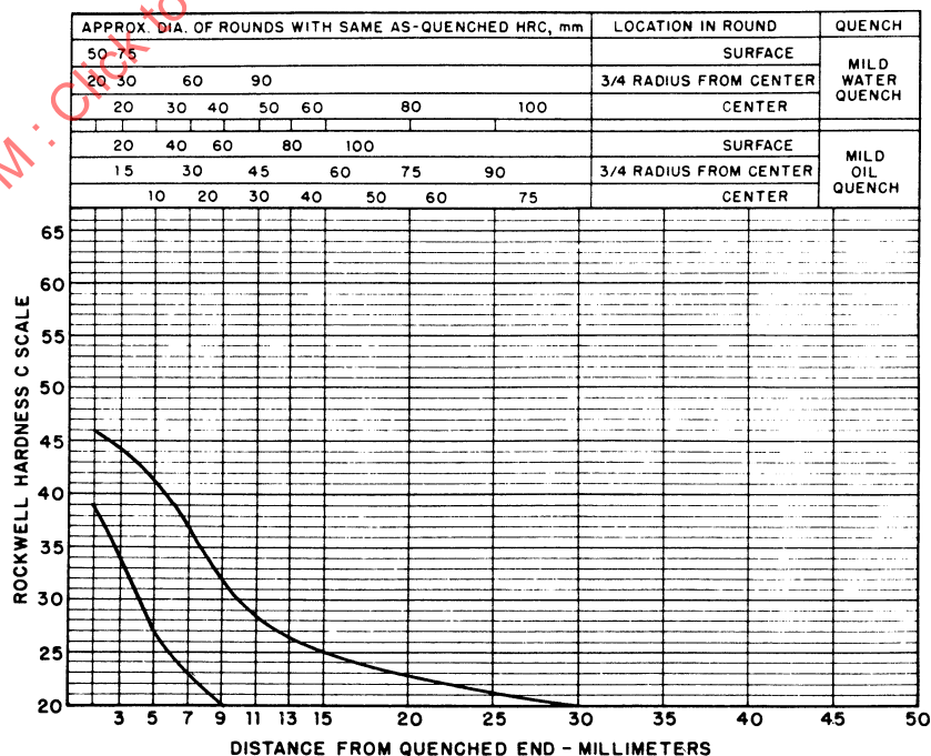
FIGURE 65—UNS H86170—HARDENABILITY BAND—SAE 8617H
