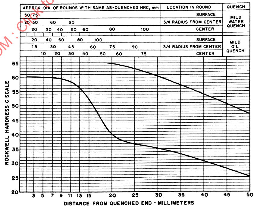
FIGURE 61—UNS H51601—HARDENABILITY BAND—SAE 51B60H
