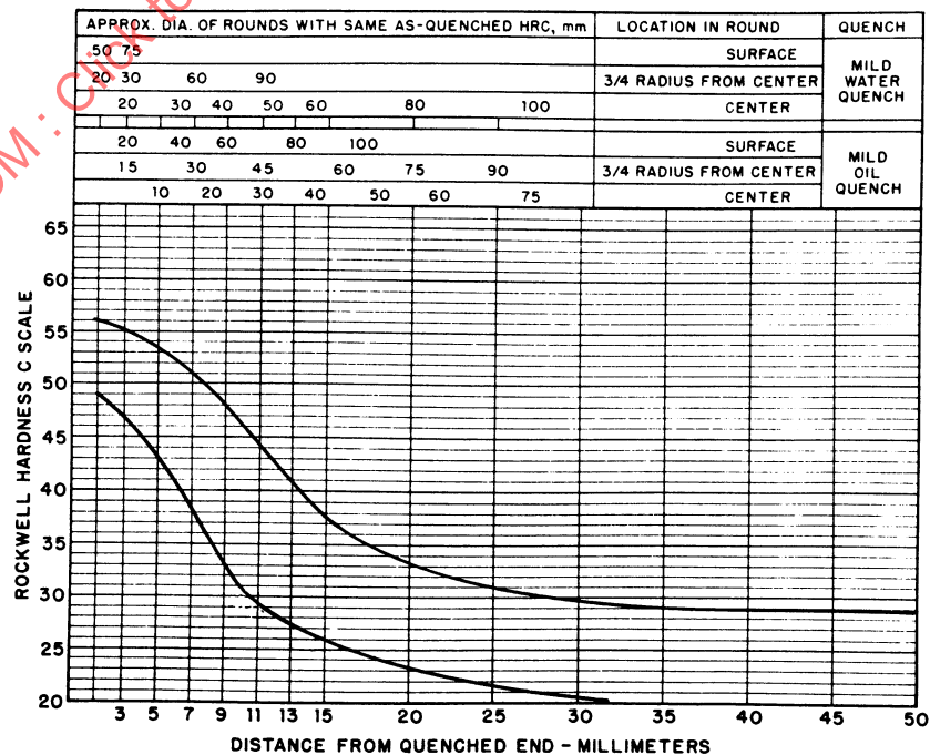
FIGURE 70—UNS H86300—HARDENABILITY BAND—SAE 8630H
