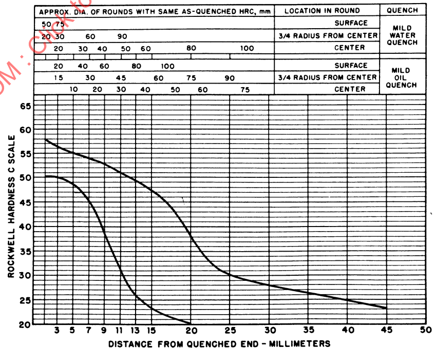
FIGURE 13—UNS H15371—HARDENABILITY BAND—SAE 15B37H
