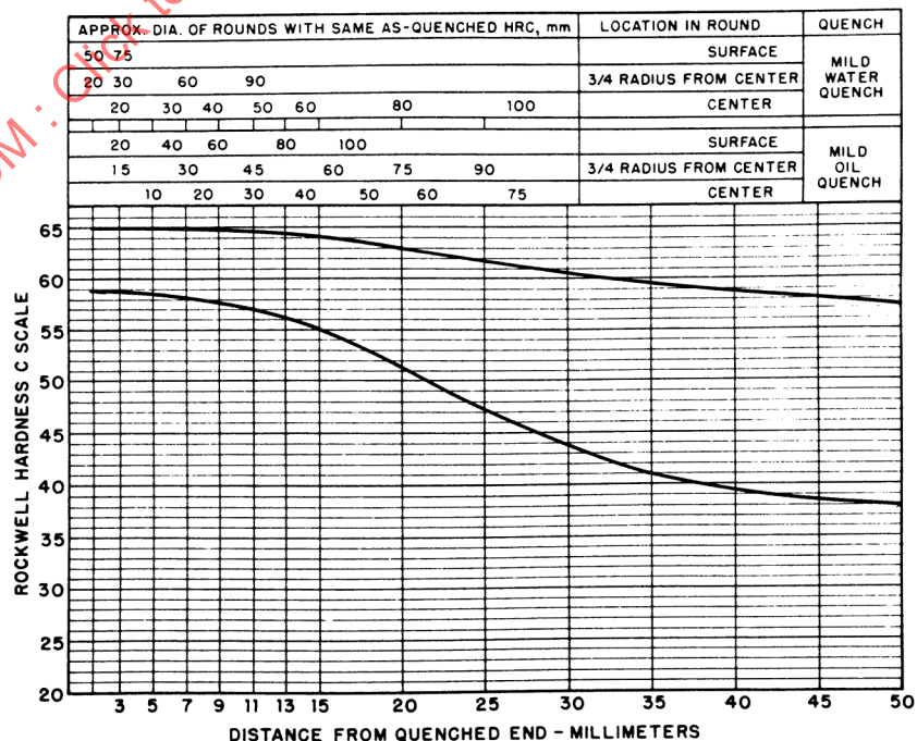
FIGURE 35—UNS H41500—HARDENABILITY BAND—SAE 4150H
