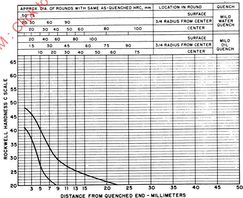
FIGURE 26—UNS H41180—HARDENABILITY BAND—SAE 4118H
