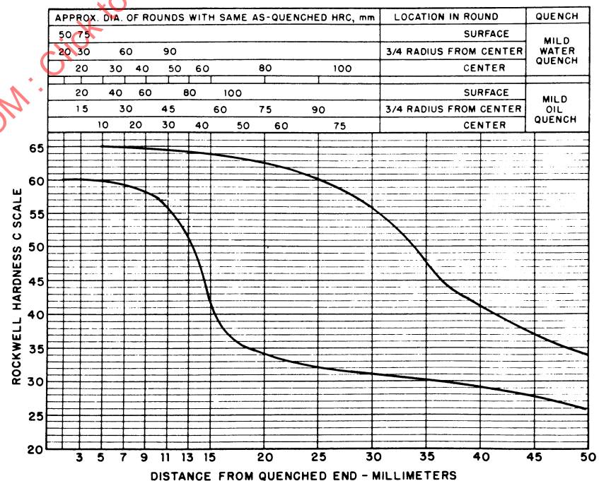
FIGURE 16—UNS H15621—HARDENABILITY BNAD—SAE 15B62H
