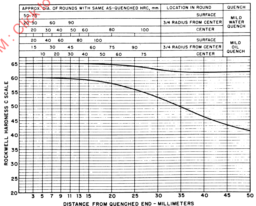
FIGURE 36—UNS H41610—HARDENABILITY BAND—SAE 4161H
