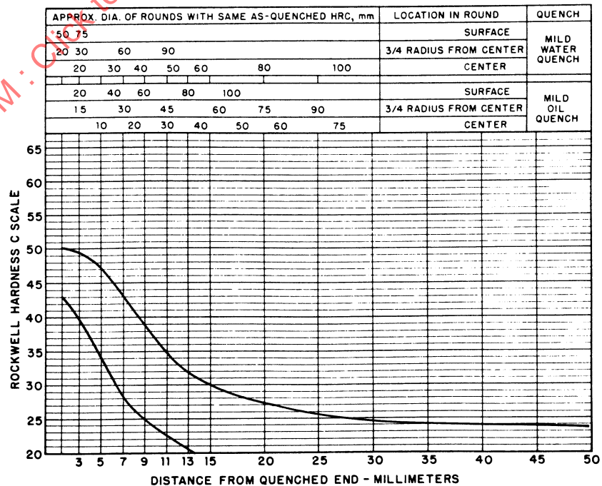
FIGURE 67—UNS H86220—HARDENABILITY BAND—SAE 8622H
