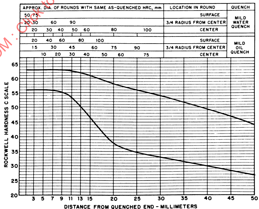
FIGURE 64—UNS H81451—HARDENABILITY BAND—SAE 81B45H
