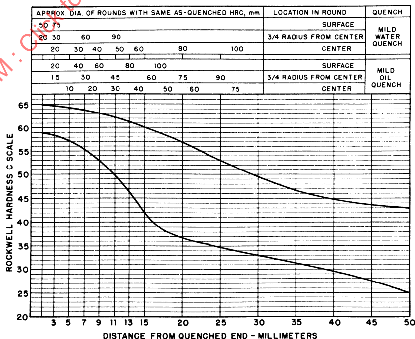
FIGURE 63—UNS H61500—HARDENABILITY BAND—SAE 6150H
