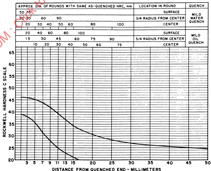
FIGURE 44—UNS H48170—HARDENABILITY BAND—SAE 4817H
