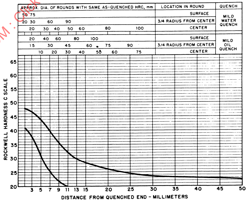
FIGURE 27—UNS H41200—HARDENABILITY BAND—SAE 4120H
