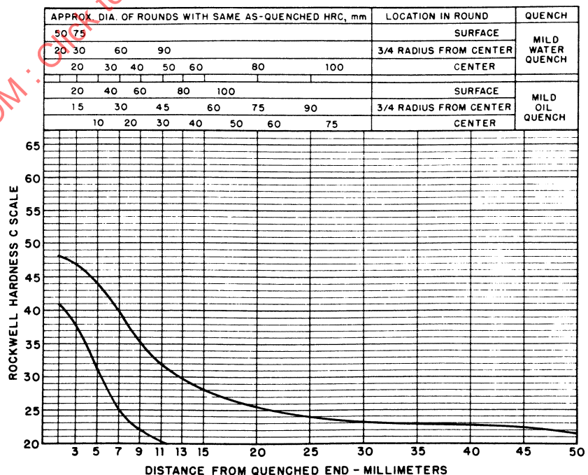
FIGURE 66—UNS H86200—HARDENABILITY BAND—SAE 8620H
