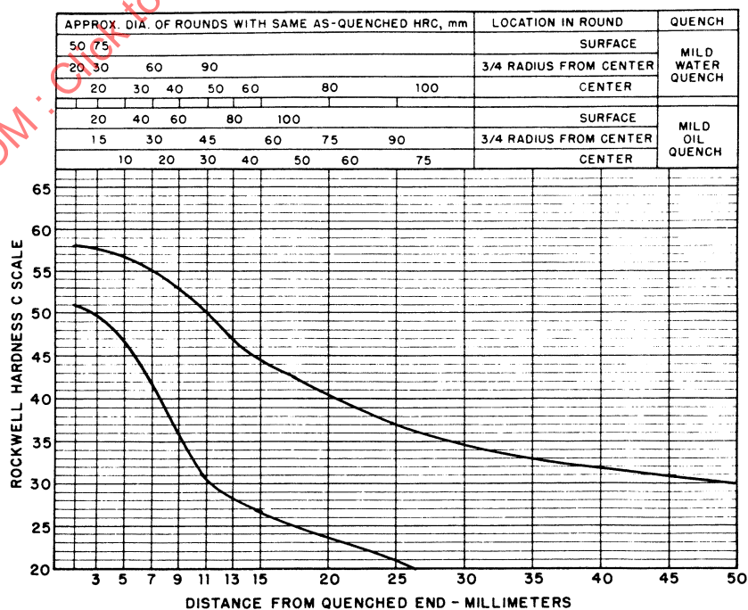
FIGURE 18—UNS H13350—HARDENABILITY BAND—SAE 1335H
