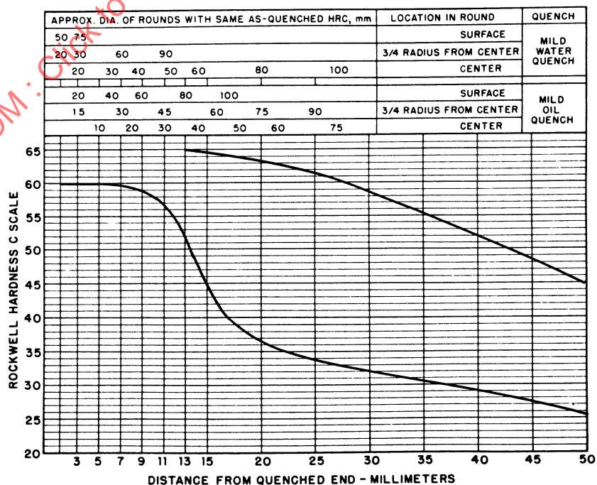
FIGURE 51—UNS H50601—HARDENABILITY BAND—SAE 50B60H
