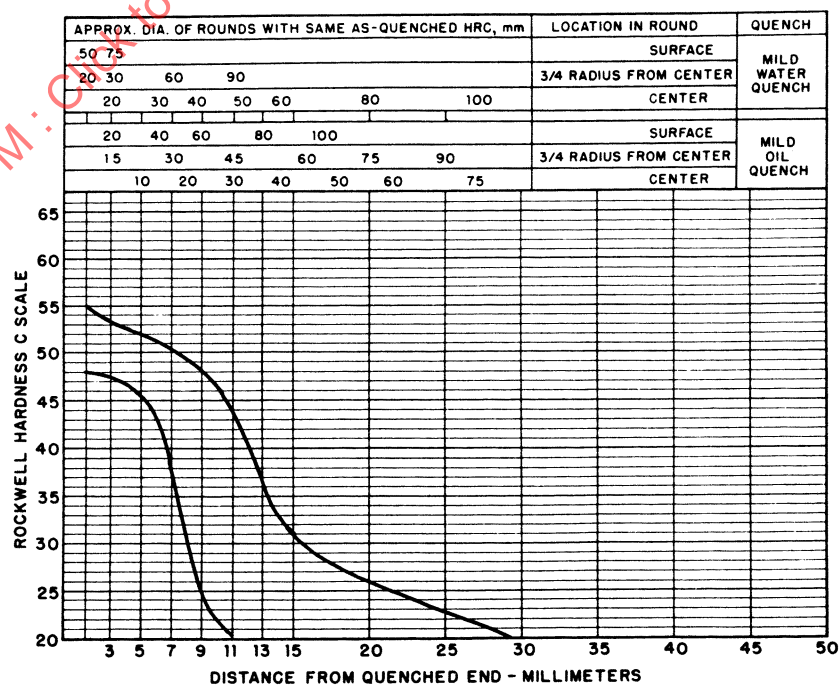
FIGURE 11—UNS H15301—HARDENABILITY BAND—SAE 15B30H
