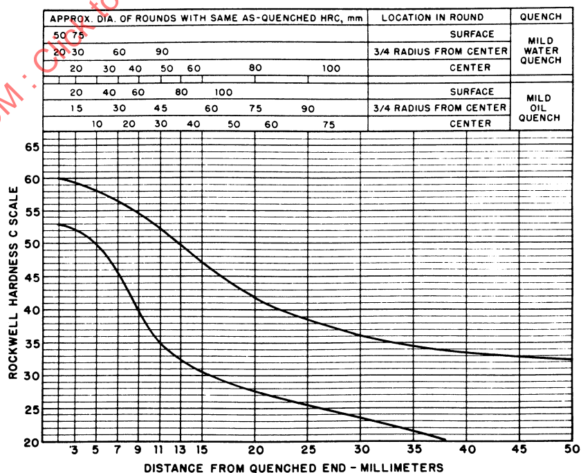
FIGURE 56—UNS H51400—HARDENABILITY BAND—SAE 5140H
