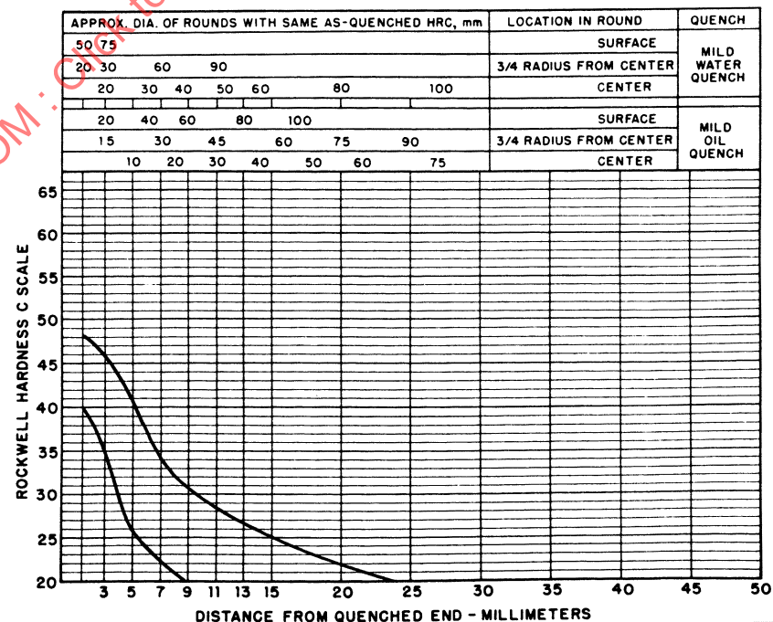
FIGURE 52—UNS H51200—HARDENABILITY BAND—SAE 5120H
