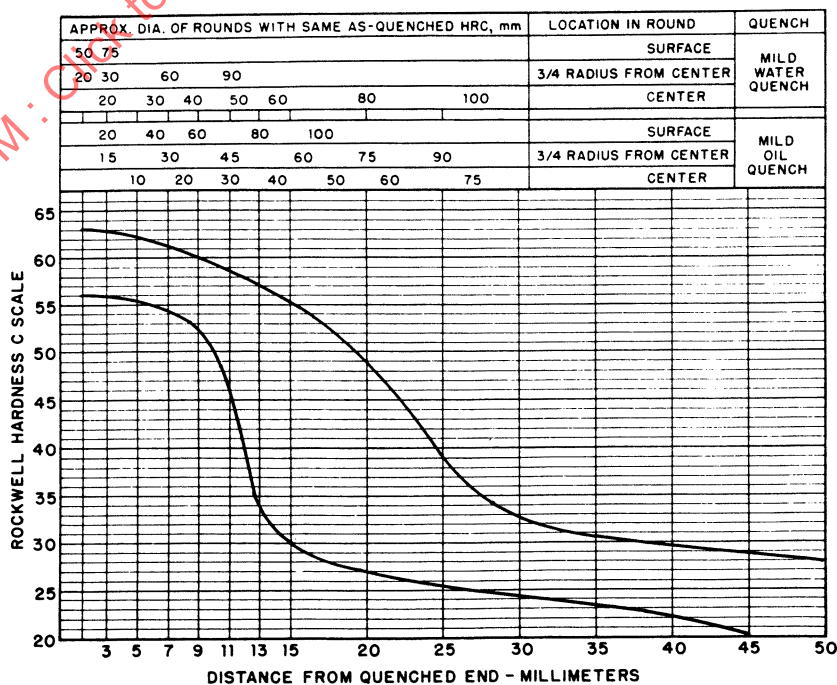
FIGURE 15—UNS H15481—HARDENABILITY BAND—SAE 15B48H
