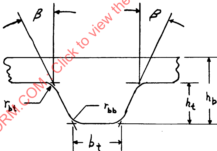
FIG. 3--BELT SECTION
