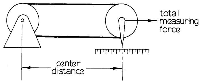
FIG. 4--DIAGRAM OF FIXTURE FOR DETERMINING BELT PITCH LENGTH
