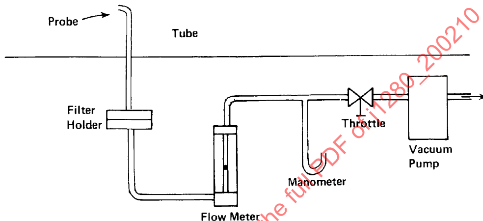
FIGURE 12—FILTER SAMPLE COLLECTION SYSTEM F
