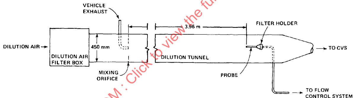
FIGURE 10—DYNAMIC DILUTION SYSTEM D
