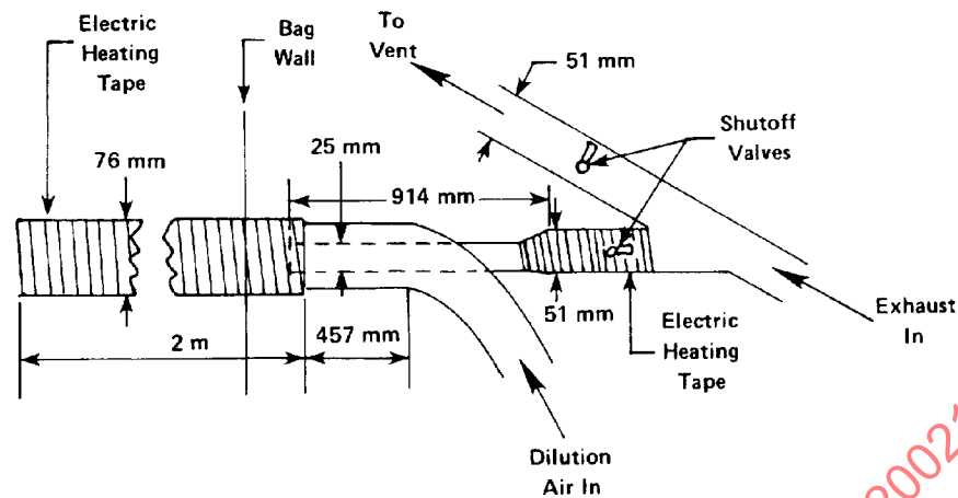
FIGURE 11—SCHEMATIC OF CONNECTOR
