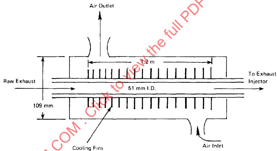
FIGURE 5—FINNED-TUBE COOLER
