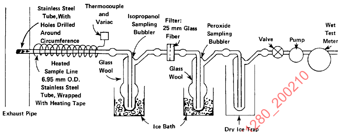
FIGURE 16—BUBBLER COLLECTION SYSTEM J
