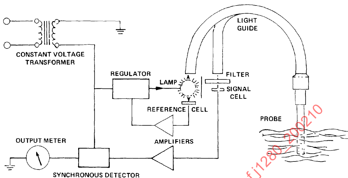
FIGURE 18—BLOCK DIAGRAM OF THE COLORIMETER AND PROBE
