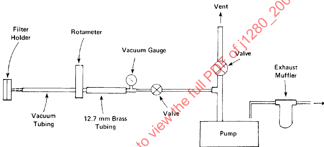
FIGURE 14—COLLECTION SYSTEM H
