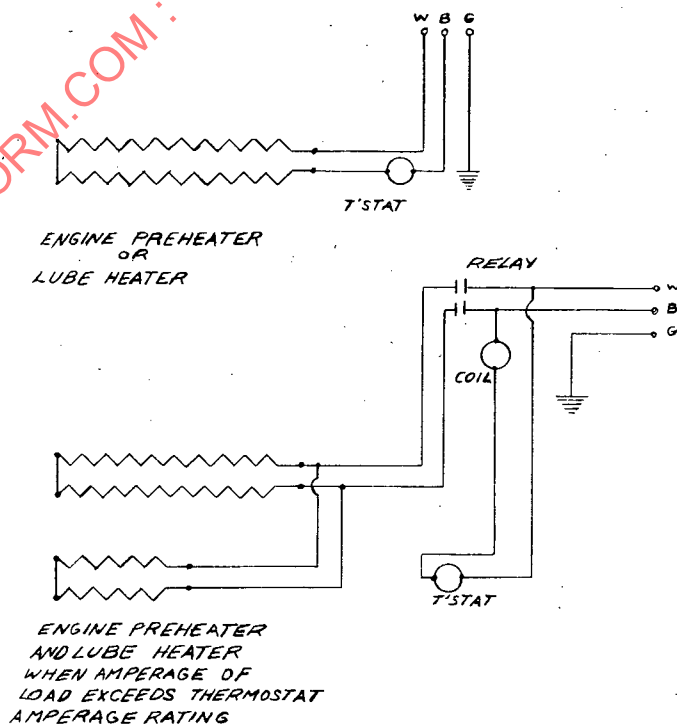
FIG. A2-TYPICAL WIRING DIAGRAMS
