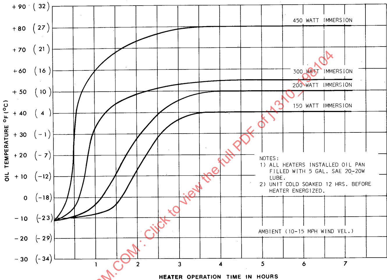
FIG. A4—TEMPERATURE RISE CURVE—OIL PAN HEATER INSTALLED IN TYPICAL DIESEL ENGINE
