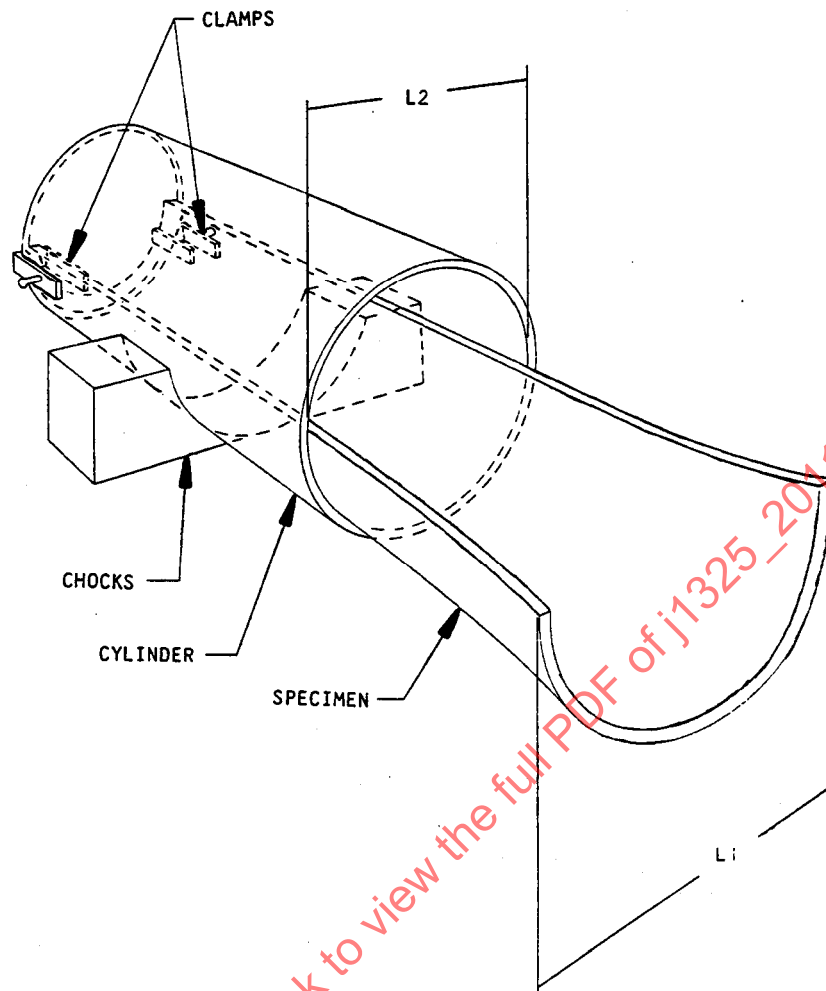
FIGURE 1—DRAPEABILITY APPARATUS
