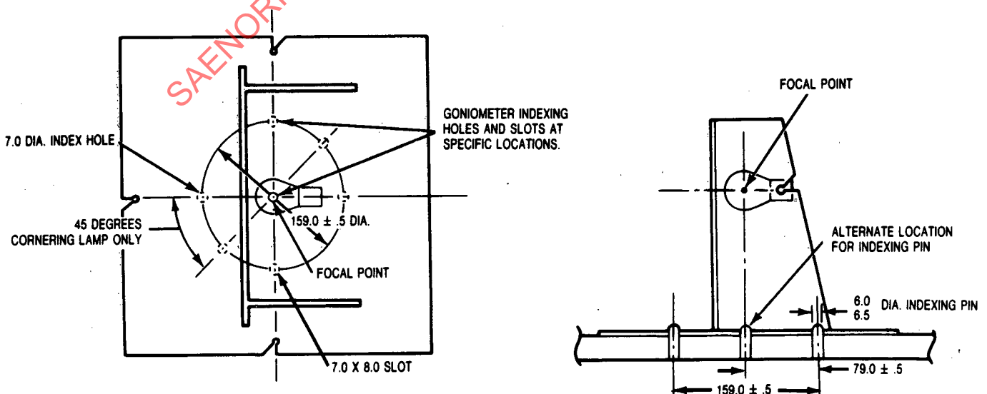
FIG. A-1—LAMP TEST FIXTURE DESIGN
