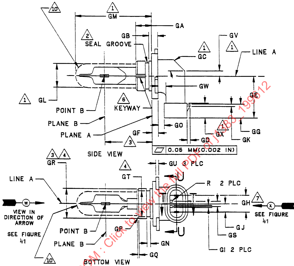
FIGURE 39A—SPECIFICATION FOR THE 9005 REPLACEABLE BULB
