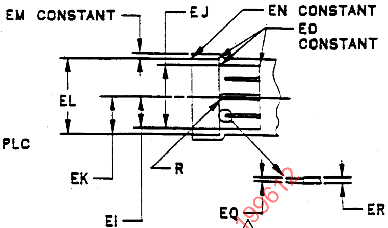
SECTION R-R (FROM FIGURE 47)
