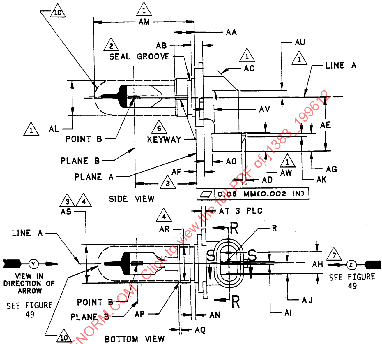
FIGURE 47A—SPECIFICATION FOR THE 9006 REPLACEABLE BULB
