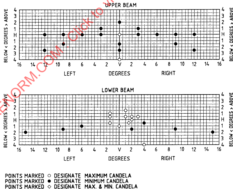
FIGURE 1—PHOTOMETRIC TABLES
