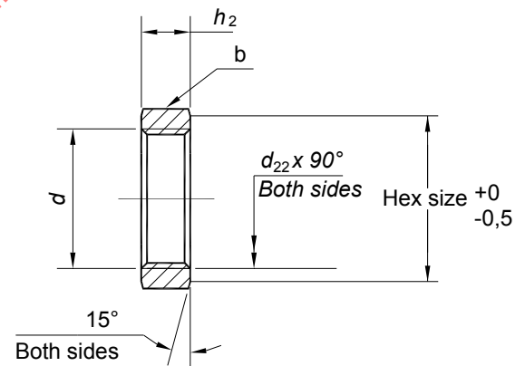
FIGURE 11 - BULKHEAD LOCKNUT
