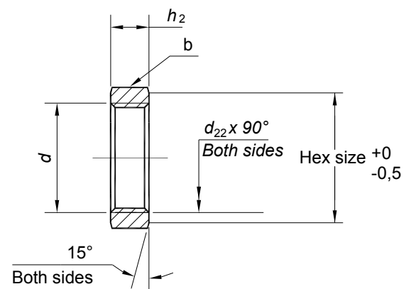
FIGURE 11 - BULKHEAD LOCKNUT
