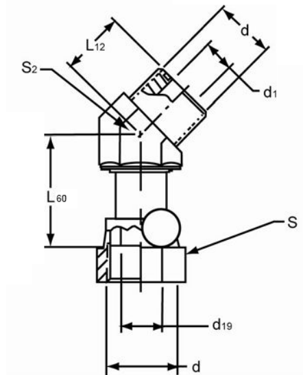
Figure 36 - Swivel 45 degree elbow (52M0321)
