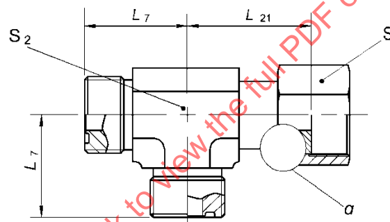
Figure 37 - Swivel run tee (52M0432)
