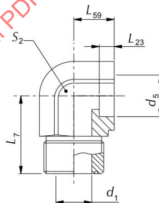
Figure 49 – Braze-on 90° male tube (52M0373 & 52M03M73)
