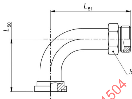
Figure 47B (Short – 52M1461 OR 52M1462) (Medium – 52M2061 OR 52M2062) (Long – 52M1561 OR 52M1562)
