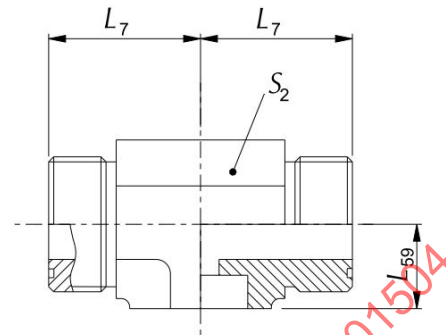
Figure 51– Braze—on male tube branch tee ( 52M0484 & 52M04M84)
