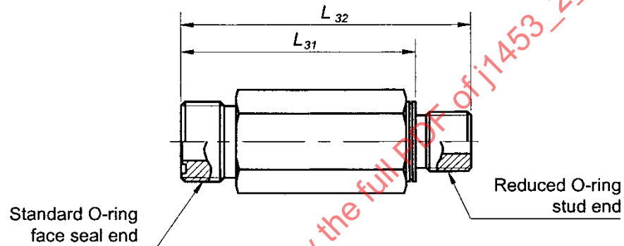
Figure A4B - Long straight stud connector with reduced stud end
