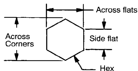
Figure 7 - Hex details
