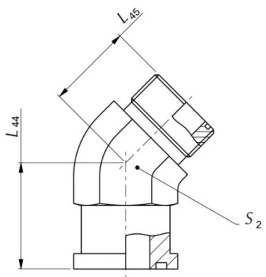
Figure 46A (Compact – 52M3361 OR 52M3362)
