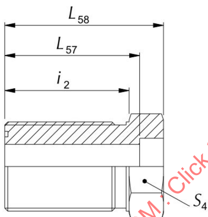
Figure 48 – Braze-on bulkhead male tube (52M0173 & 52M01M73)
