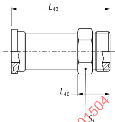
Figure 44B (Short – 52M3061 OR 52M3062) (Medium – 52M3161 OR 52M3162) (Long – 52M3261 OR 52M3262)
