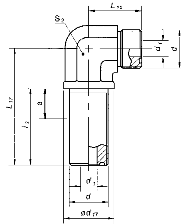
Figure 25 - 90 Degree bulkhead elbow (52M0701)
