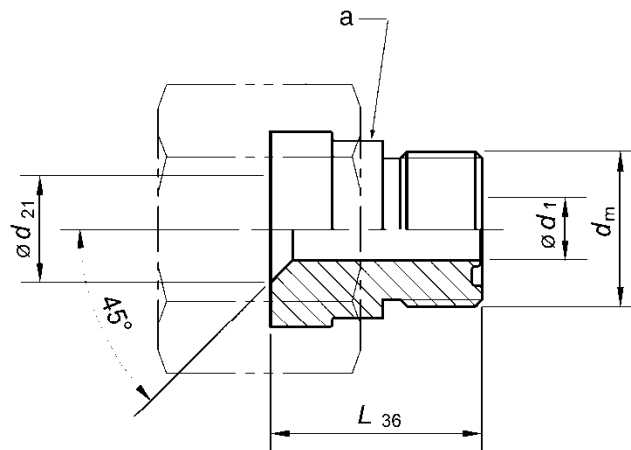
Figure 44 - Reducer without nut (Style B) (520123B)
