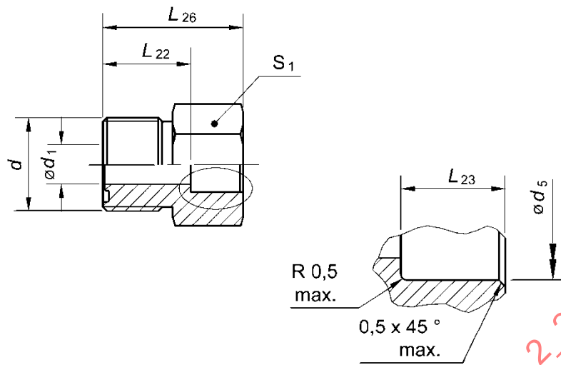
Figure 40 - Braze-on straight (52M0172), (52M01M72, metric tubing)
