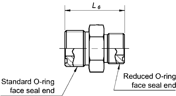
Figure A5 - Straight union connector with one end reduced
