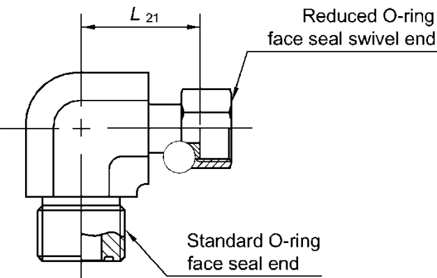
Figure A6 - Swivel elbow connector with reduced swivel end
