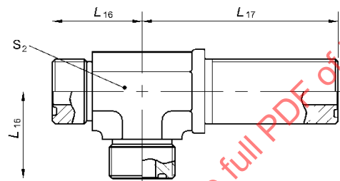
Figure 26 - Bulkhead run tee (52M0958)
