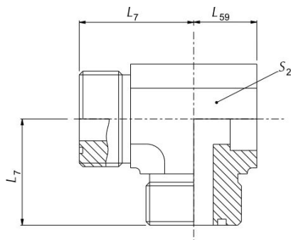
Figure 50 – Braze-on male tube run tee adapter ( 52M0483 & 52m04M83)
