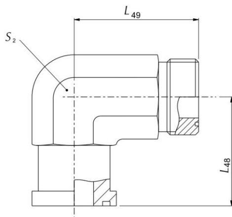
Figure 47A (Compact – 52M3461 OR 52M3462)
