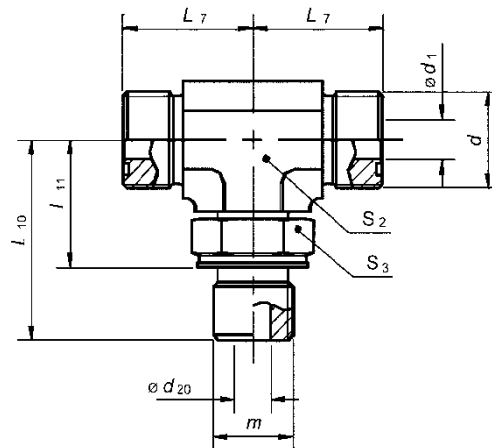
Figure 18 - Adjustable stud branch tee (52M0489)
