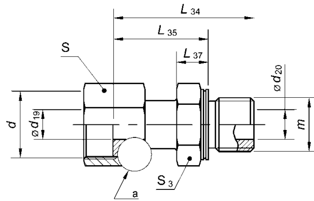
Figure 39 - Stud straight swivel (52M0196)
