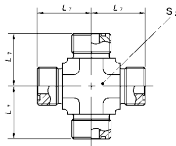
Figure 33 - Union cross (52M0501)
