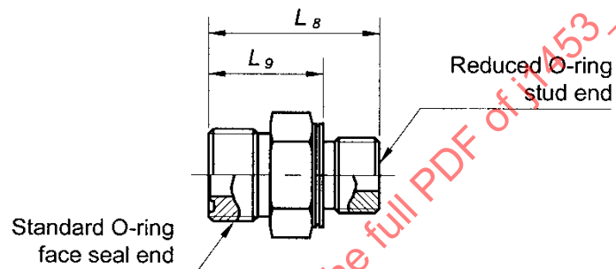
Figure A3B - Straight-stud connector with reduced stud end
