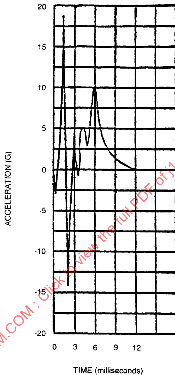
Figure 12—OPERATIONAL SHOCK PROFILE
