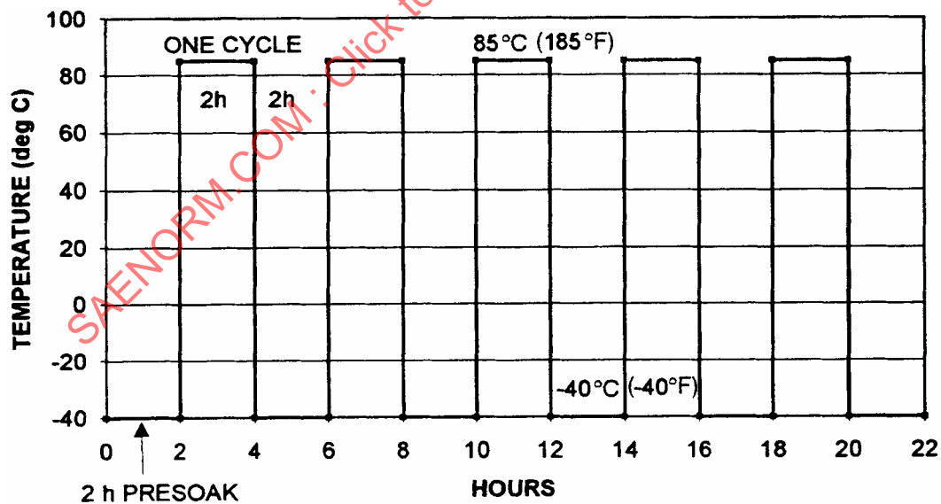
FIGURE 2C - THERMAL SHOCK
