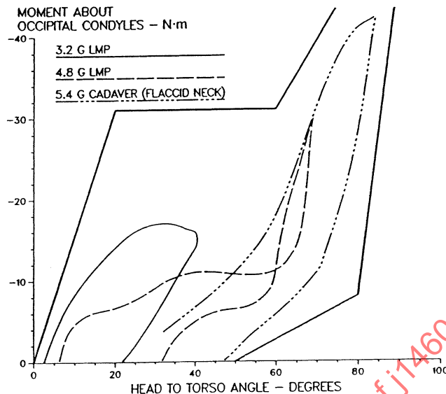
FIGURE 29—MOMENT-ANGLE NECK EXTENSION RESPONSES OF A VOLUNTEER WITH TENSED MUSCLES AND A CADAVER WITH FLACCID MUSCLES COMPARED TO THE NECK EXTENSION CORRIDOR FOR THE MID-SIZE ADULT MALE SEATED IN AUTOMOTIVE POSTURE
