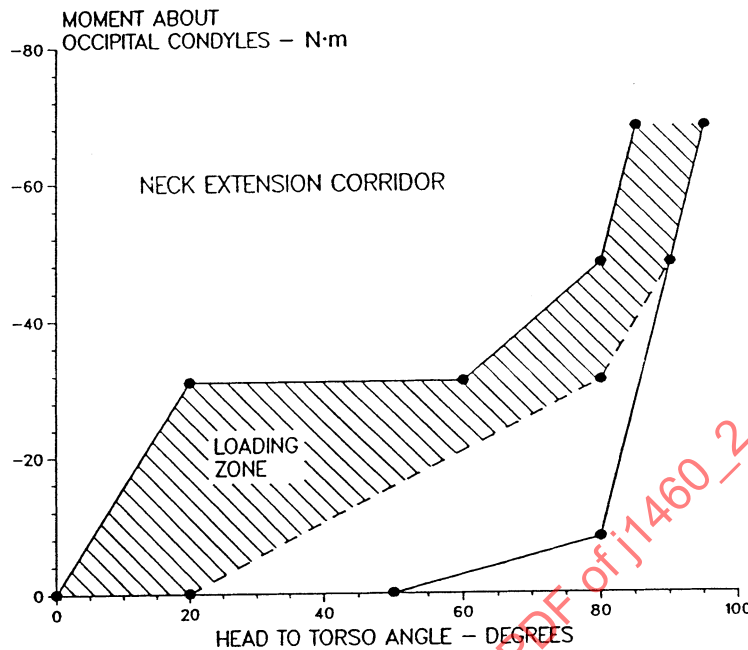
FIGURE 28—MOMENT-ANGLE NECK EXTENSION CORRIDOR AND LOADING ZONE FOR THE MID-SIZE ADULT MALE SEATED IN AUTOMOTIVE POSTURE (SEE 2.1.3.(4) AND 2.1.3.(22))
