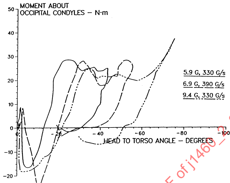
FIGURE 21—MOMENT-ANGLE NECK FLEXION RESPONSES OF VOLUNTEER SUBJECT 4 FOR VARIOUS HYGE SLED ACCELERATION AND ONSET LEVELS. TENSED NECK MUSCLES AND ERECT SEATED POSTURE (SEE 2.1.3.(8))
