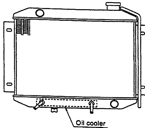
FIGURE 2 - EXAMPLE OF OIL COOLER INSTALLATION (DOWNFLOW TYPE RADIATOR)
