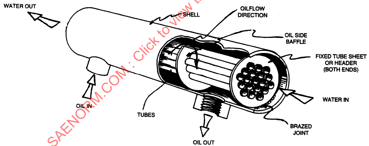
FIGURE 13 - SHELL AND TUBE OIL TO WATER COOLER-FIXED BUNDLE
