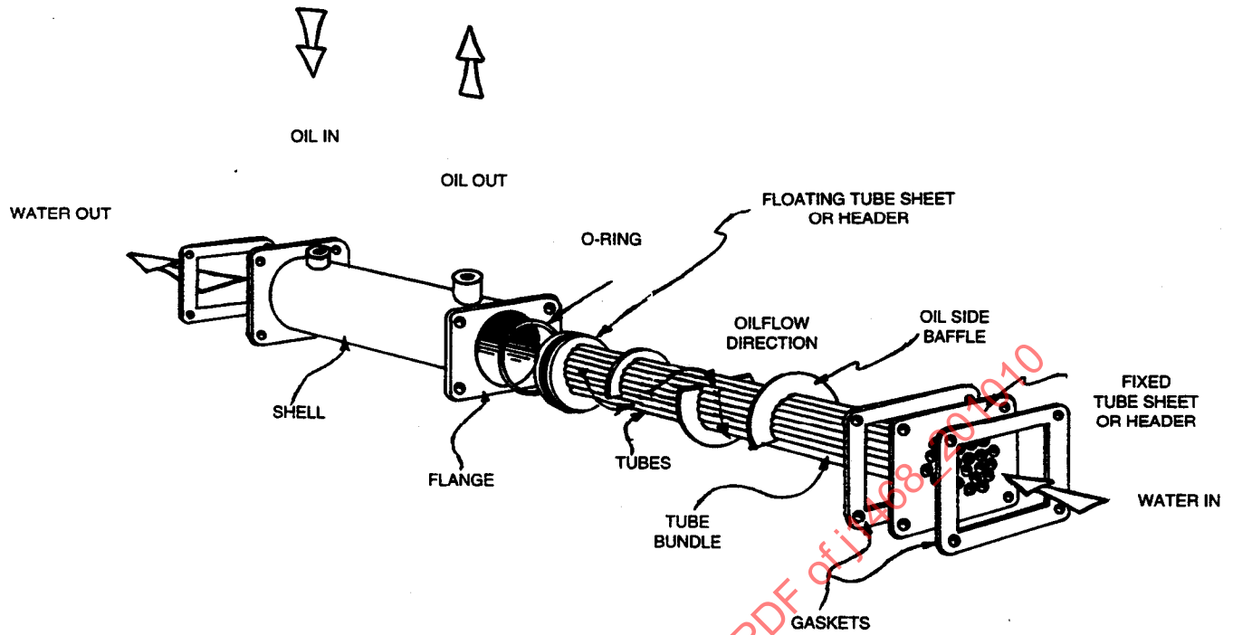
FIGURE 12 - SHELL AND TUBE REMOVABLE BUNDLE OIL TO WATER COOLER
