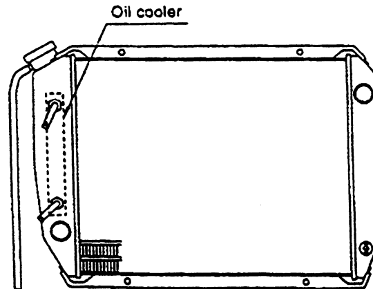
FIGURE 4 - EXAMPLE OF OIL COOLER INSTALLATION (CROSSFLOW TYPE RADIATOR)
