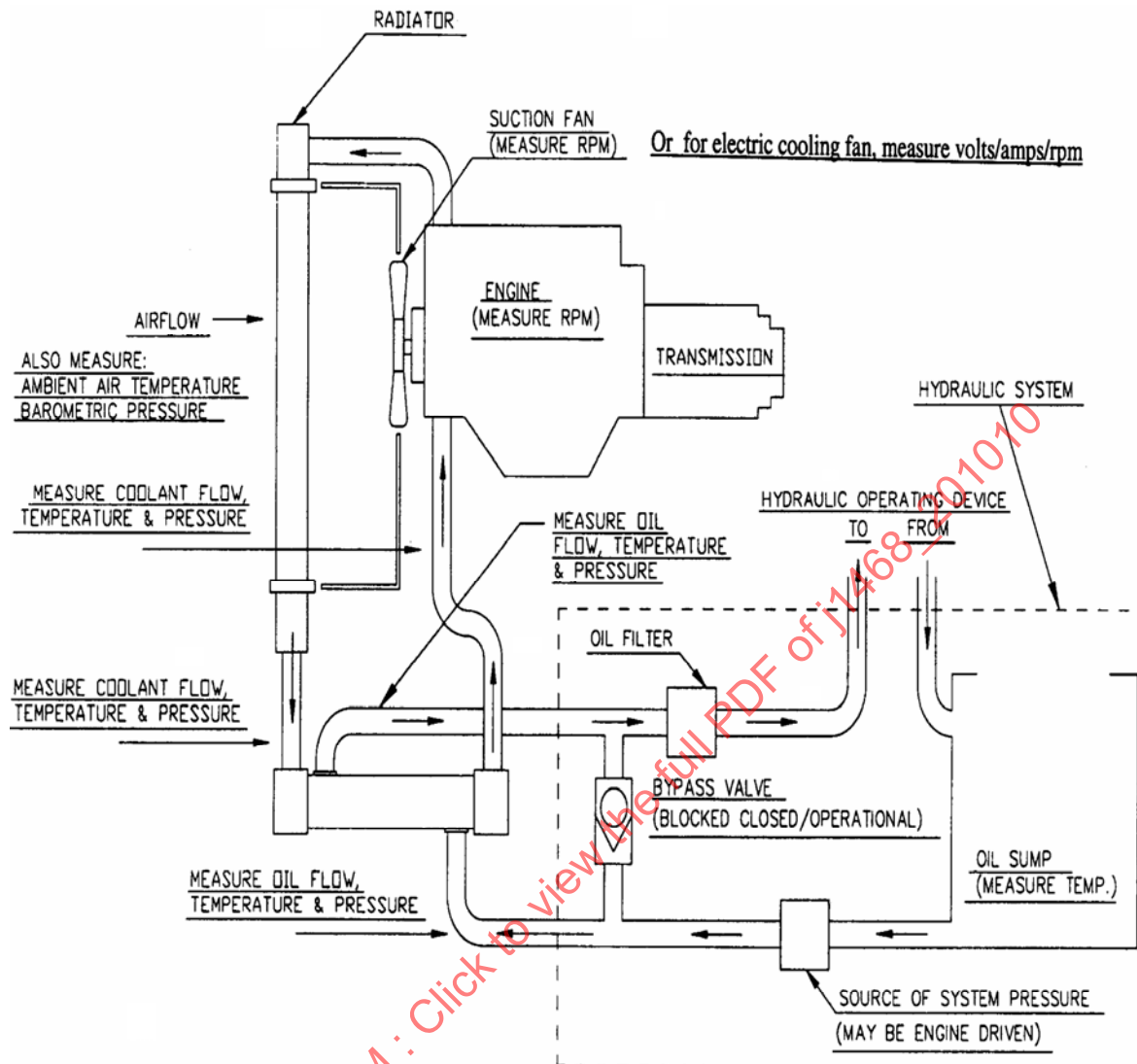
FIGURE 10 - SCHEMATIC OF TYPICAL REMOTE-MOUNTED OIL COOLER SYSTEM
