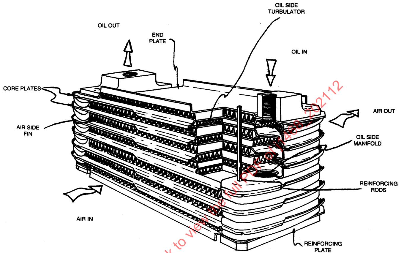
Figure 11 - Plate fin separator oil to air cooler
