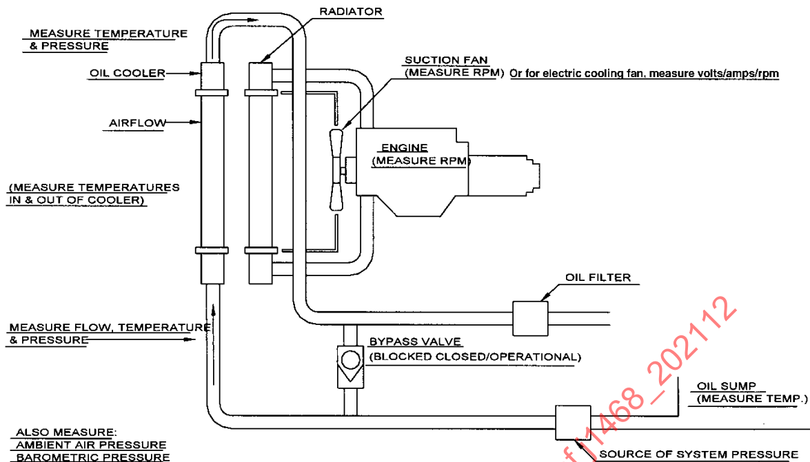
Figure 1 - Schematic of typical oil-to-air cooler system and test data required
