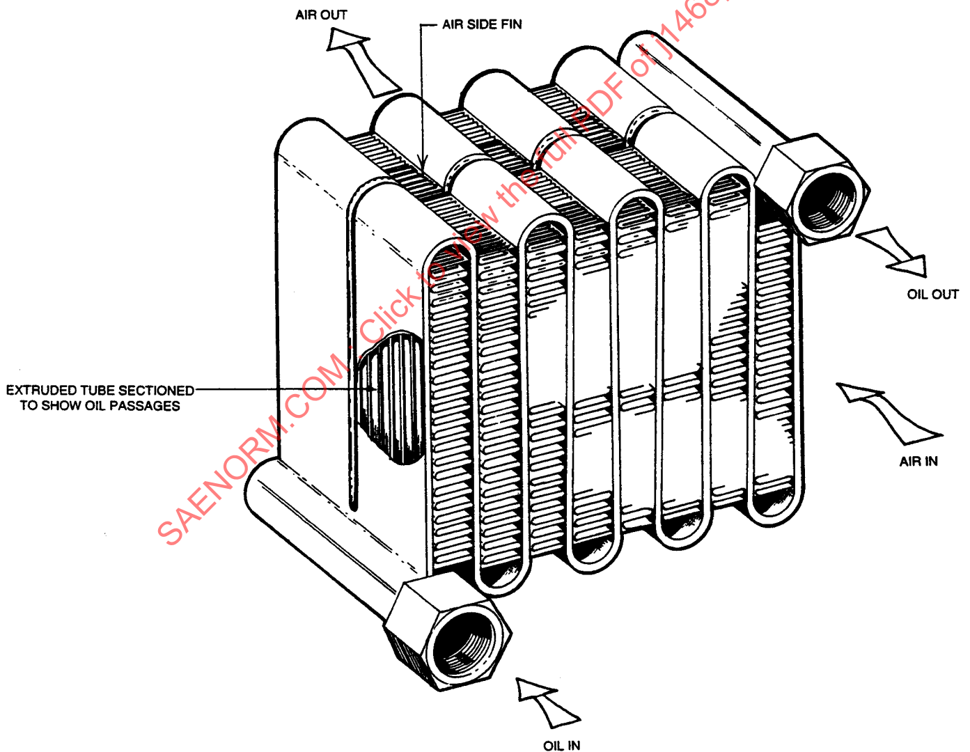
Figure 14 - Serpentine tube and fin oil to air cooler
