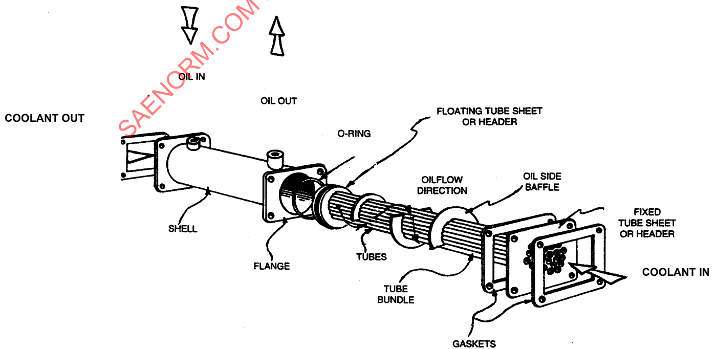
Figure 12 - Shell and tube removable bundle oil to coolant cooler
