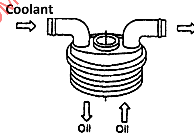
Figure 8 - Tube-in-shell direct mount oil cooler
