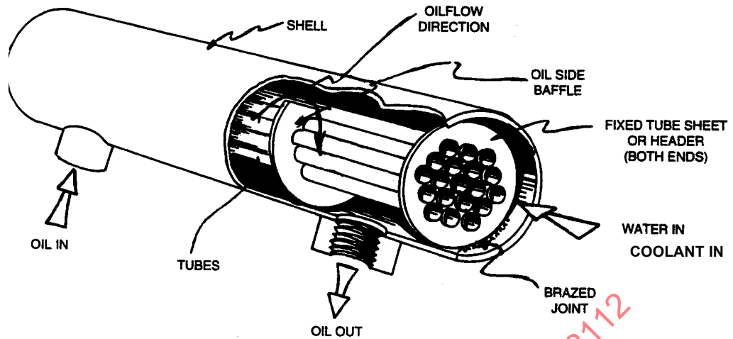
Figure 13 - Shell and tube oil to coolant cooler (fixed bundle)
