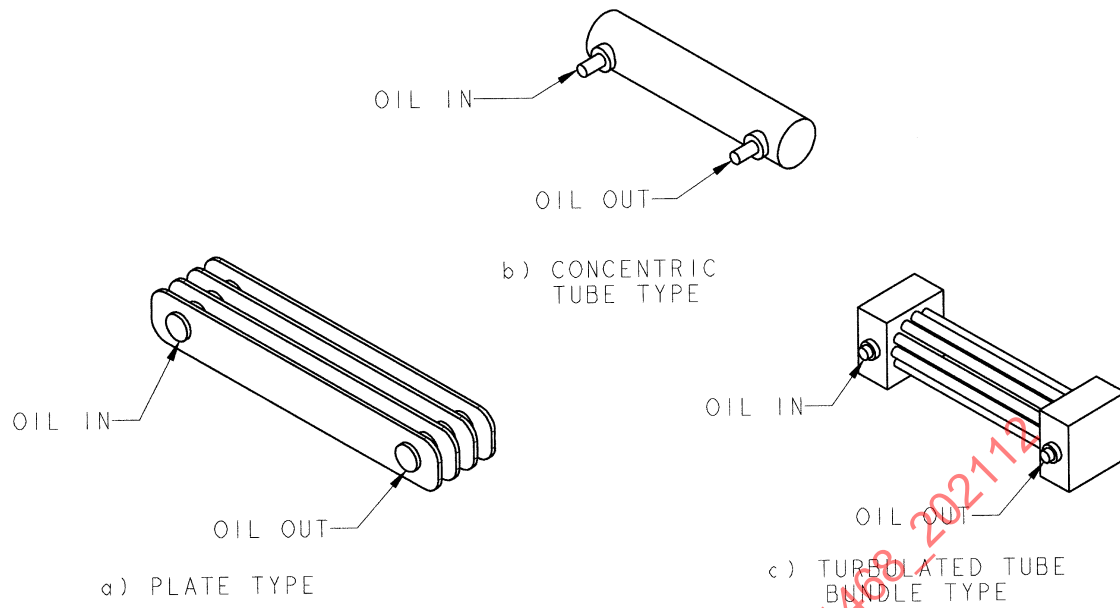
Figure 3 - Oil coolers for mounting in radiator outlet or bottom tanks
