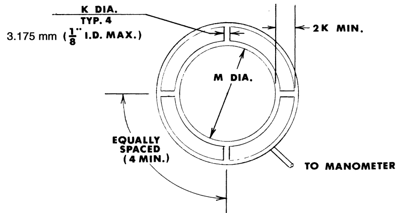
FIGURE 2 - PIEZOMETER RING
