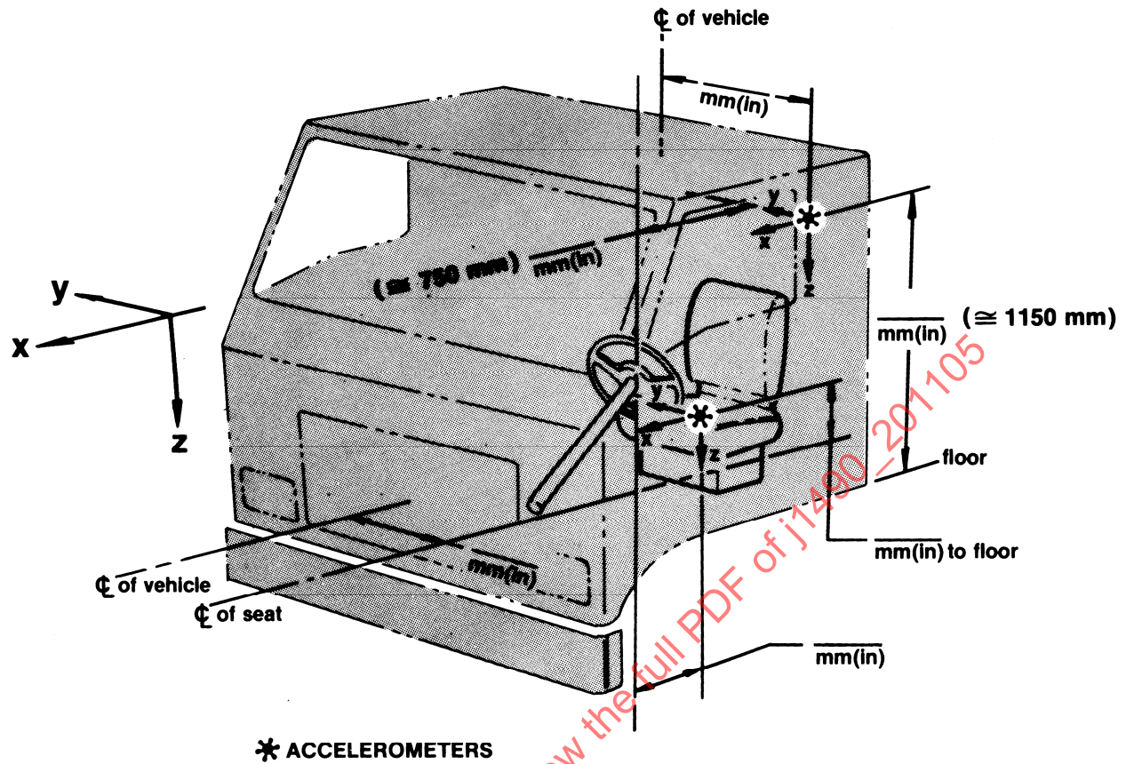
FIGURE 4C—TEST VEHICLE DESCRIPTION SHEET 3C ACCELEROMETER LOCATIONS WITHIN TEST VEHICLE CAB
