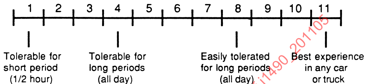
FIGURE 6A—SAMPLE SUBJECTIVE EVALUATION SCALE
