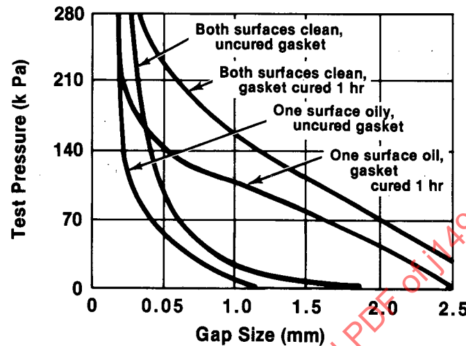
FIGURE 7 - Typical RTV Gap vs. Pressure
