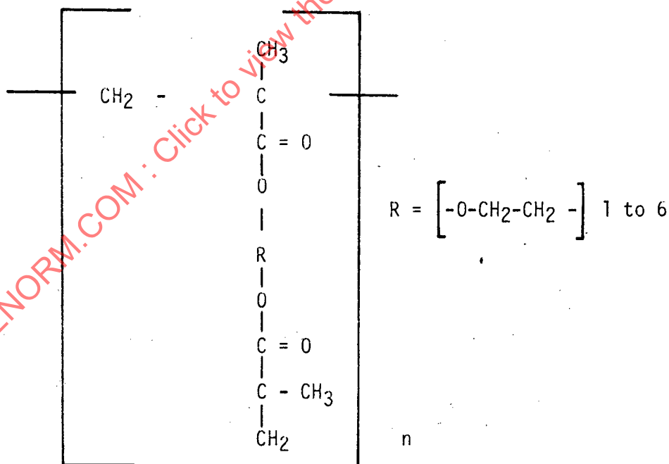
FIGURE 4 - Chemical Structure
