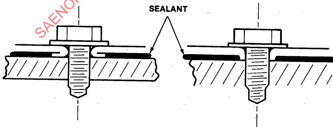
FIGURE 11 - Grooved Flange
