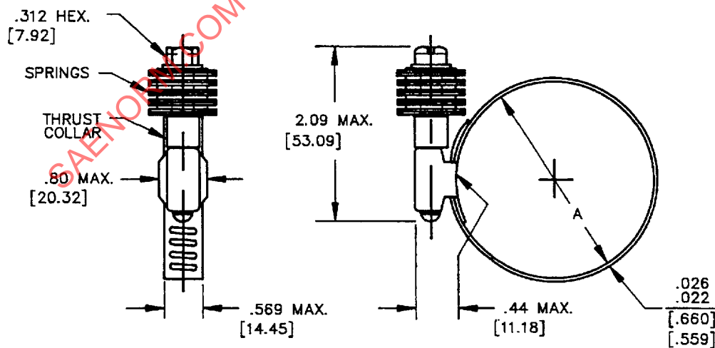
FIGURE 21—TYPE "SLF"—INCH (METRIC)
