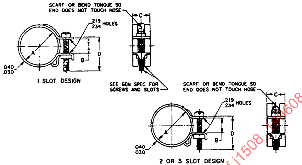
FIGURE 2—DIMENSIONS OF TYPE "B" HOSE CLAMPS
