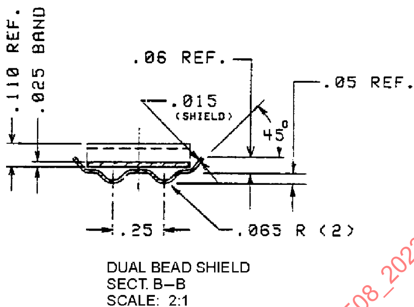
Figure 23 - Type "T," inch (metric)
