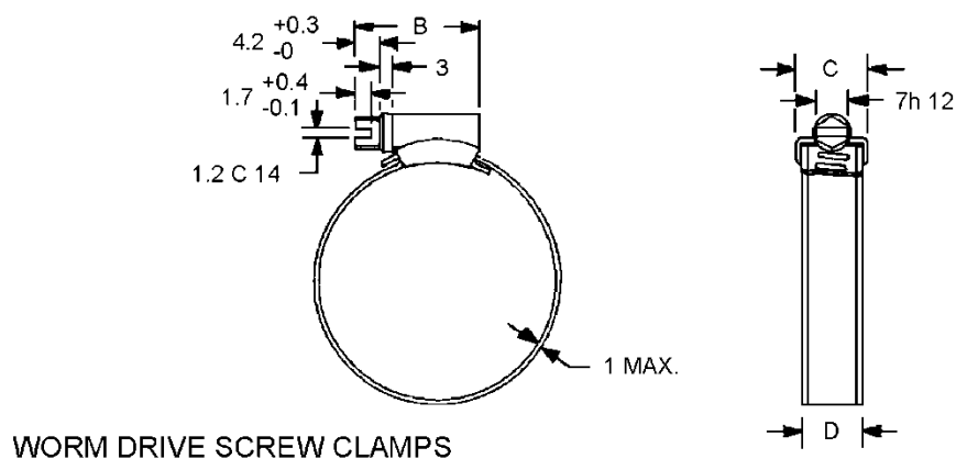
Figure 10B - Type "FE," mm
