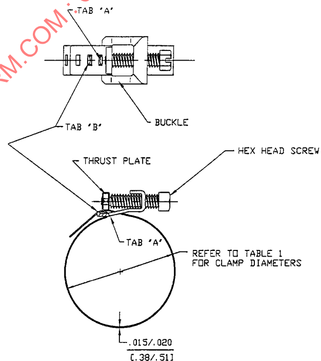
Figure 15B - Type "G," inch (metric)
