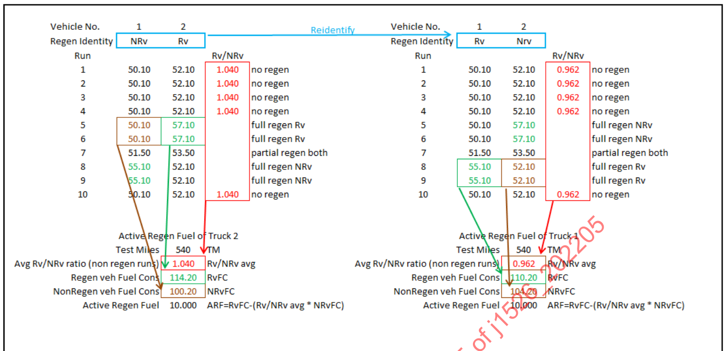
Figure B1 - Active regeneration fuel calculation example
