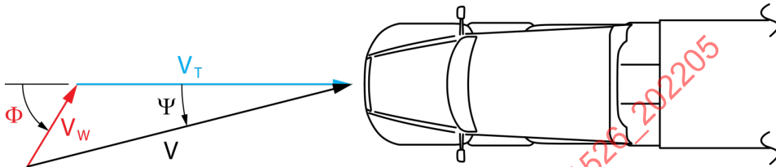
Figure A1 - Vehicle wind velocity and yaw diagram
