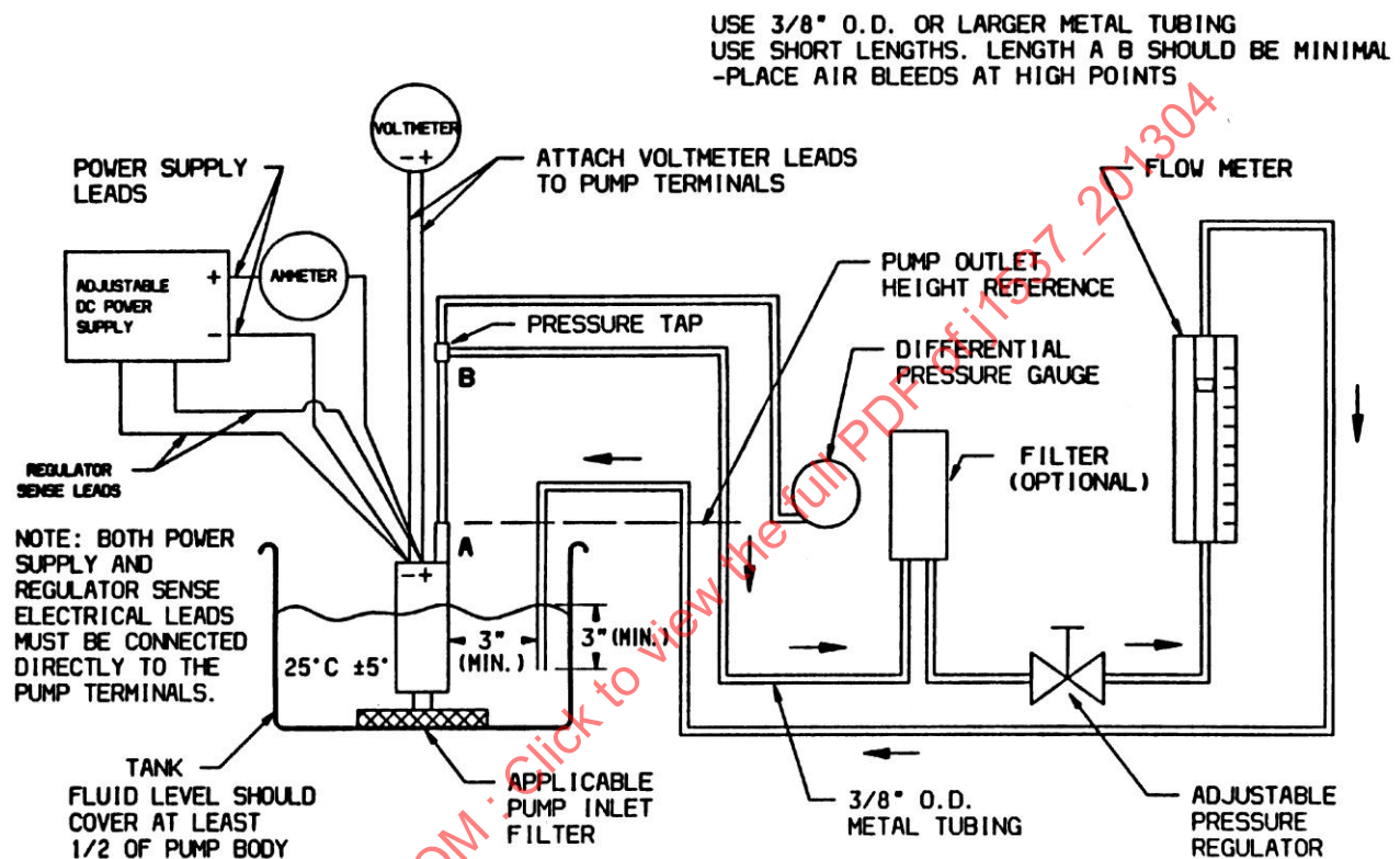
FIGURE 1—ELECTRIC FUEL PUMP FLOW PERFORMANCE TEST SET-UP
