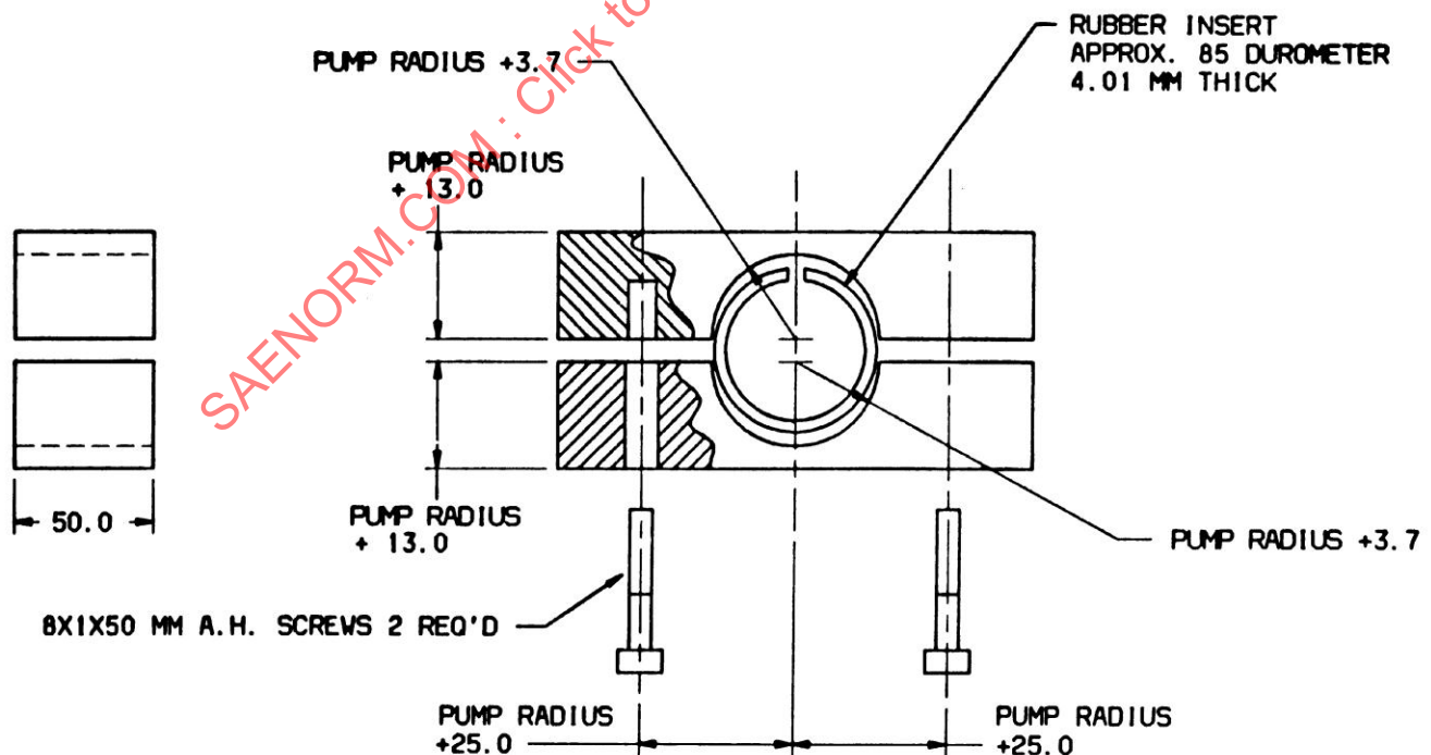
FIGURE 4—PUMP VIBRATION TEST FIXTURE TYPICAL STATION
