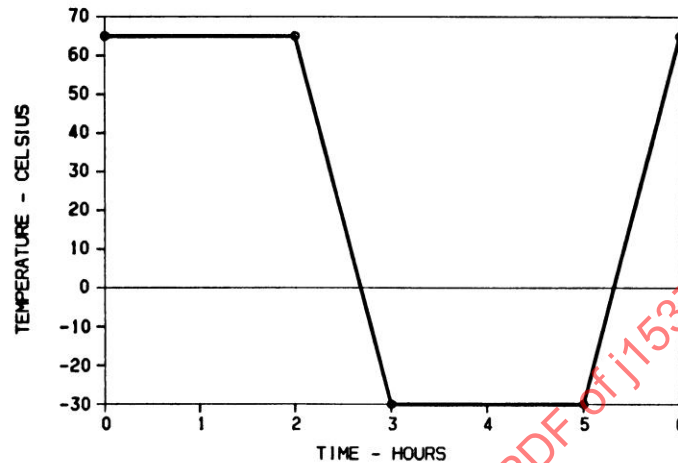
FIGURE 5—TEMPERATURE CYCLE TEST SCHEDULE
