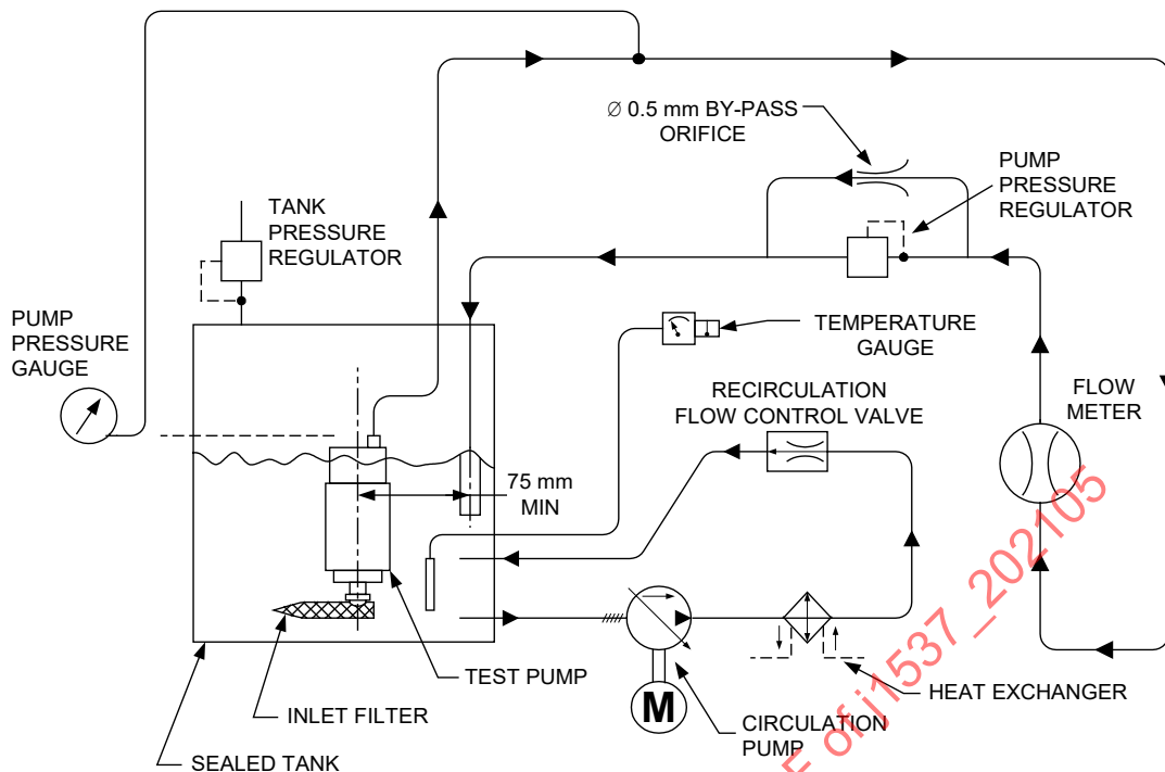
Figure 2 - Schematic of equipment for the hot fuel handling test
