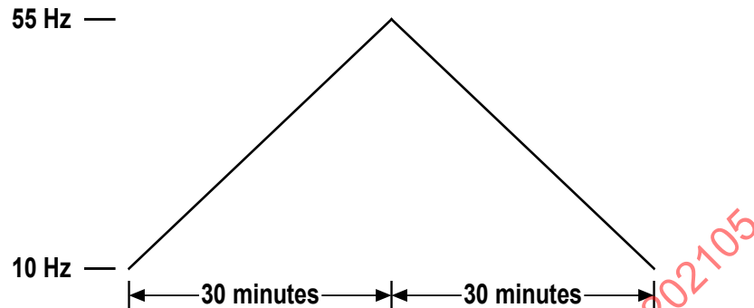
Figure 6 - Test cycle for the pump vibration forcing frequency
