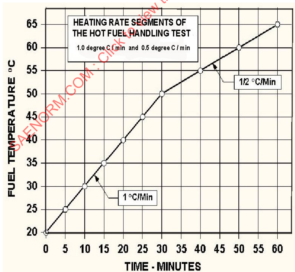
Figure 4 - Fuel heating rate for the hot fuel handling test
