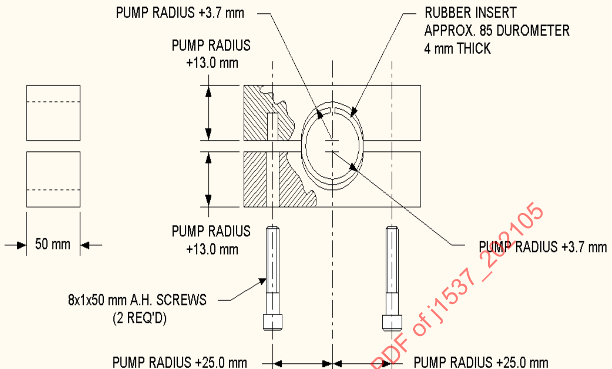
Figure 5 - Representative pump vibration test fixture
