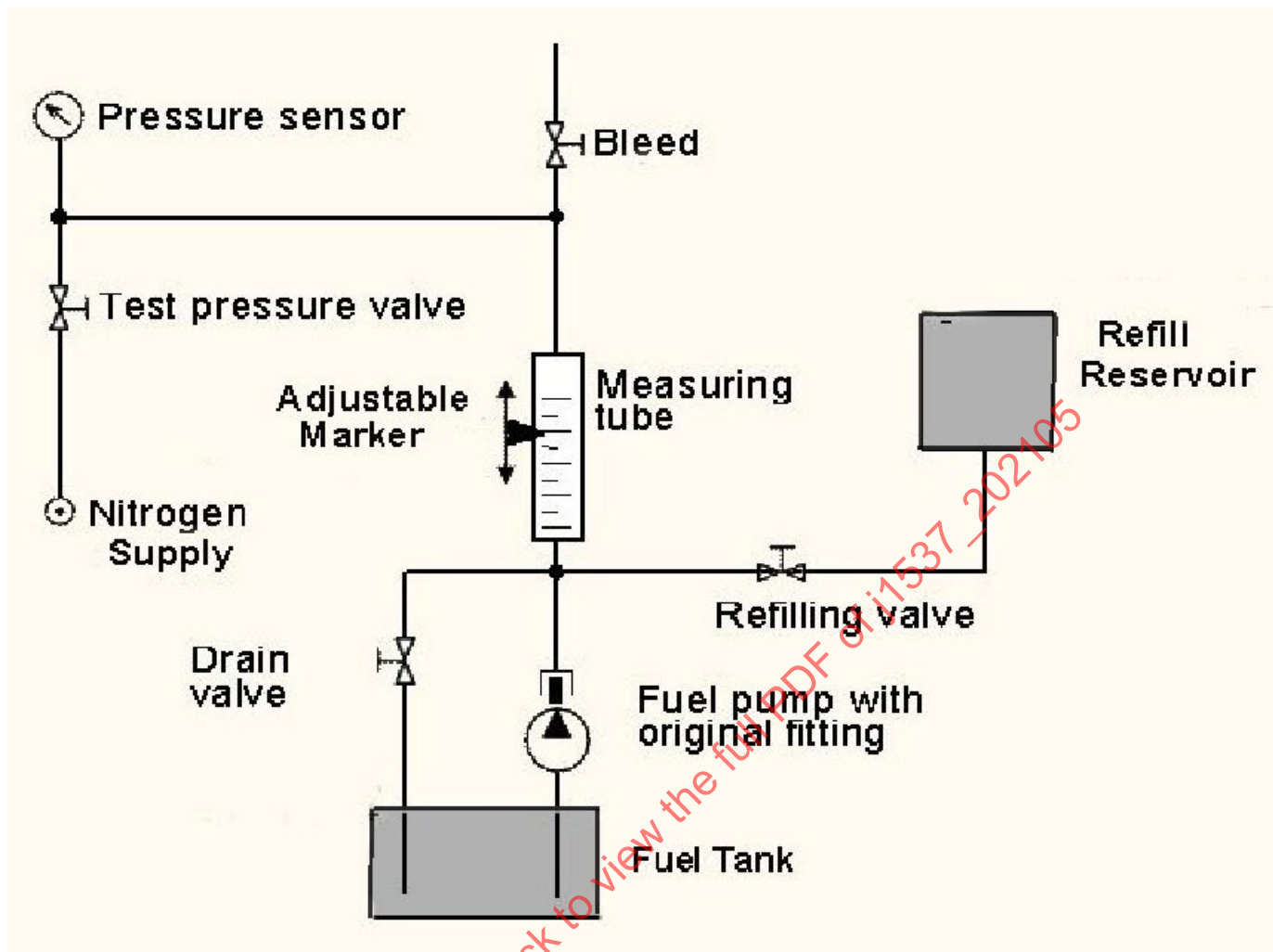
Figure 3 - Schematic of the test fixture for determining the reverse flow leakage
